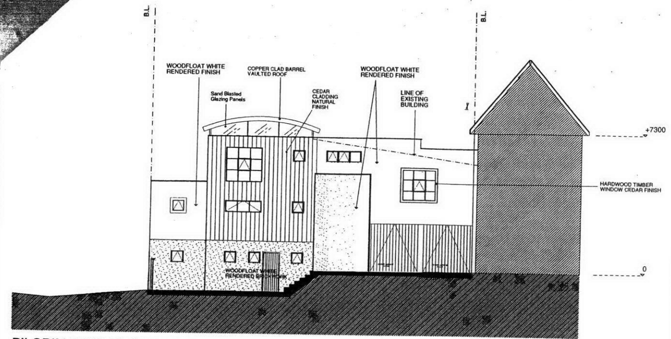
PILGRIM ROAD ELEVATION 1:100
