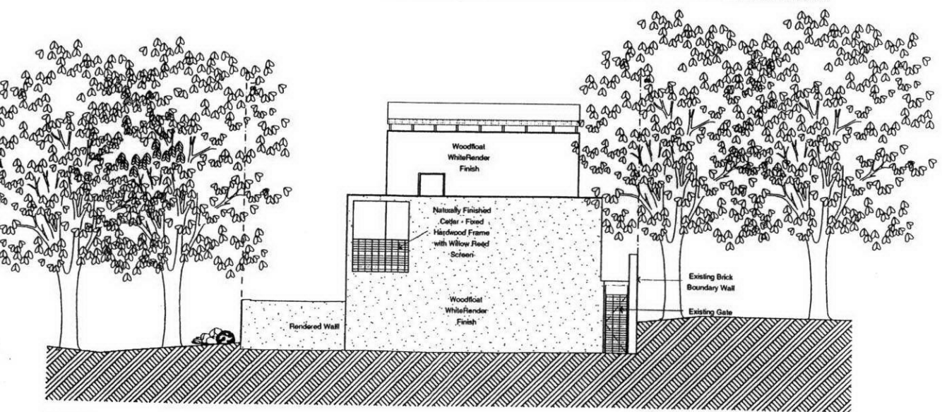
EAST ELEVATION 1:100
