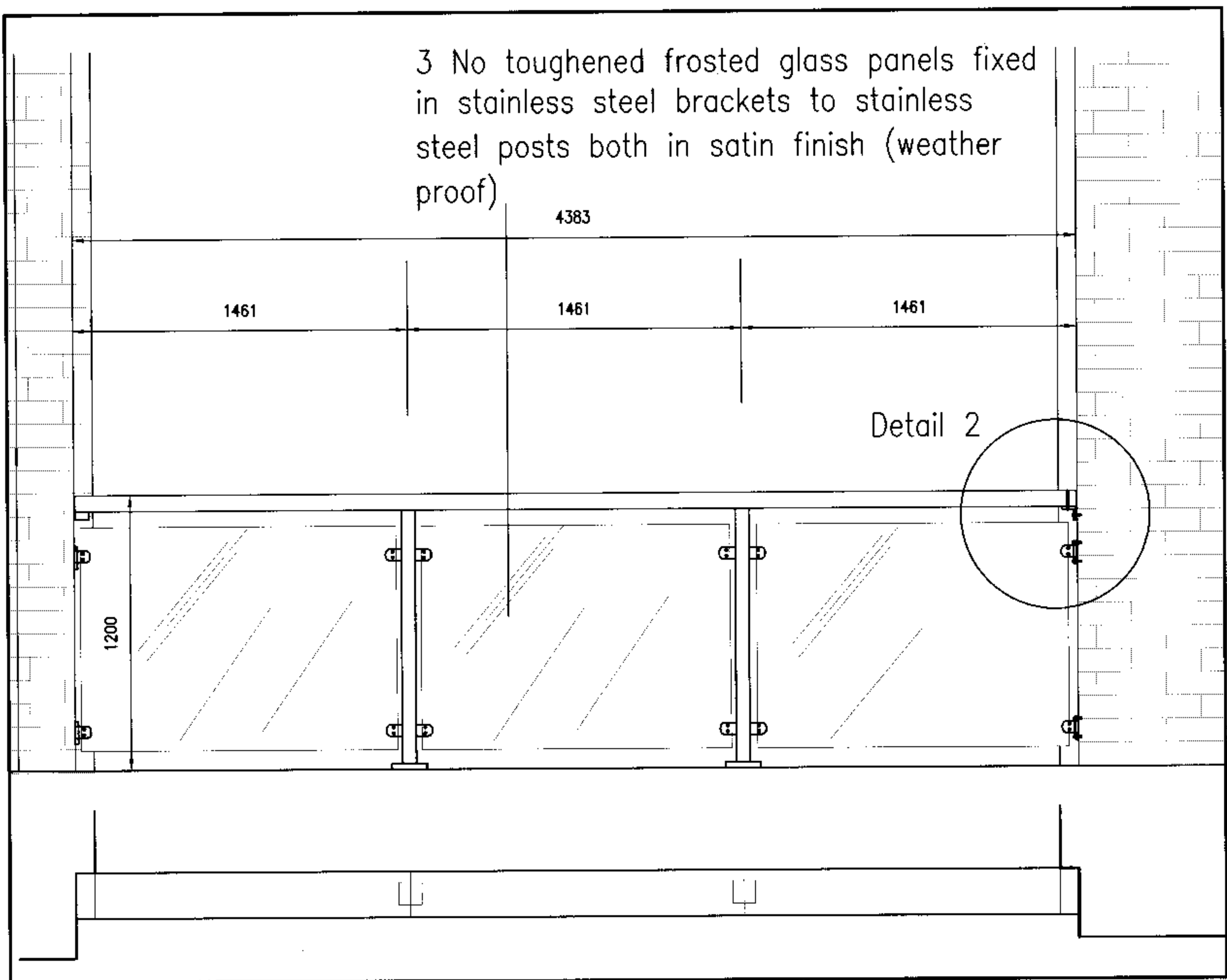
Elevation 2 Scale 1:25
