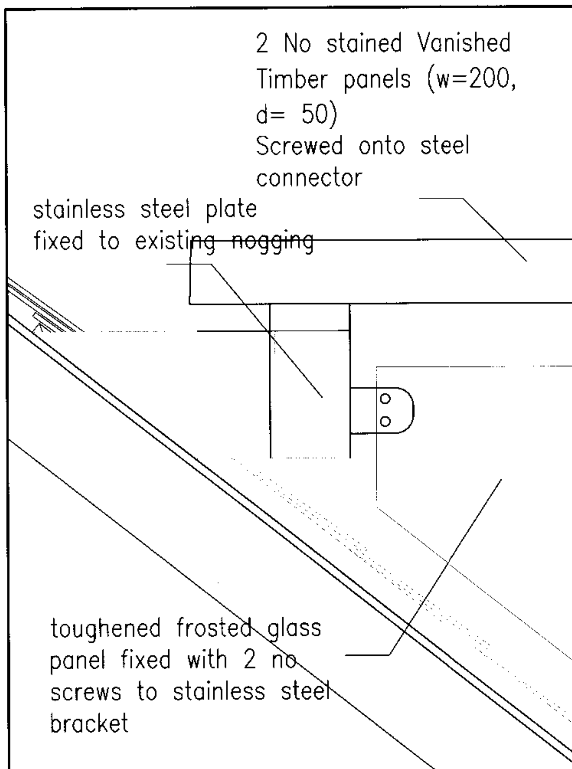
Detail 1 Scale 1:5
