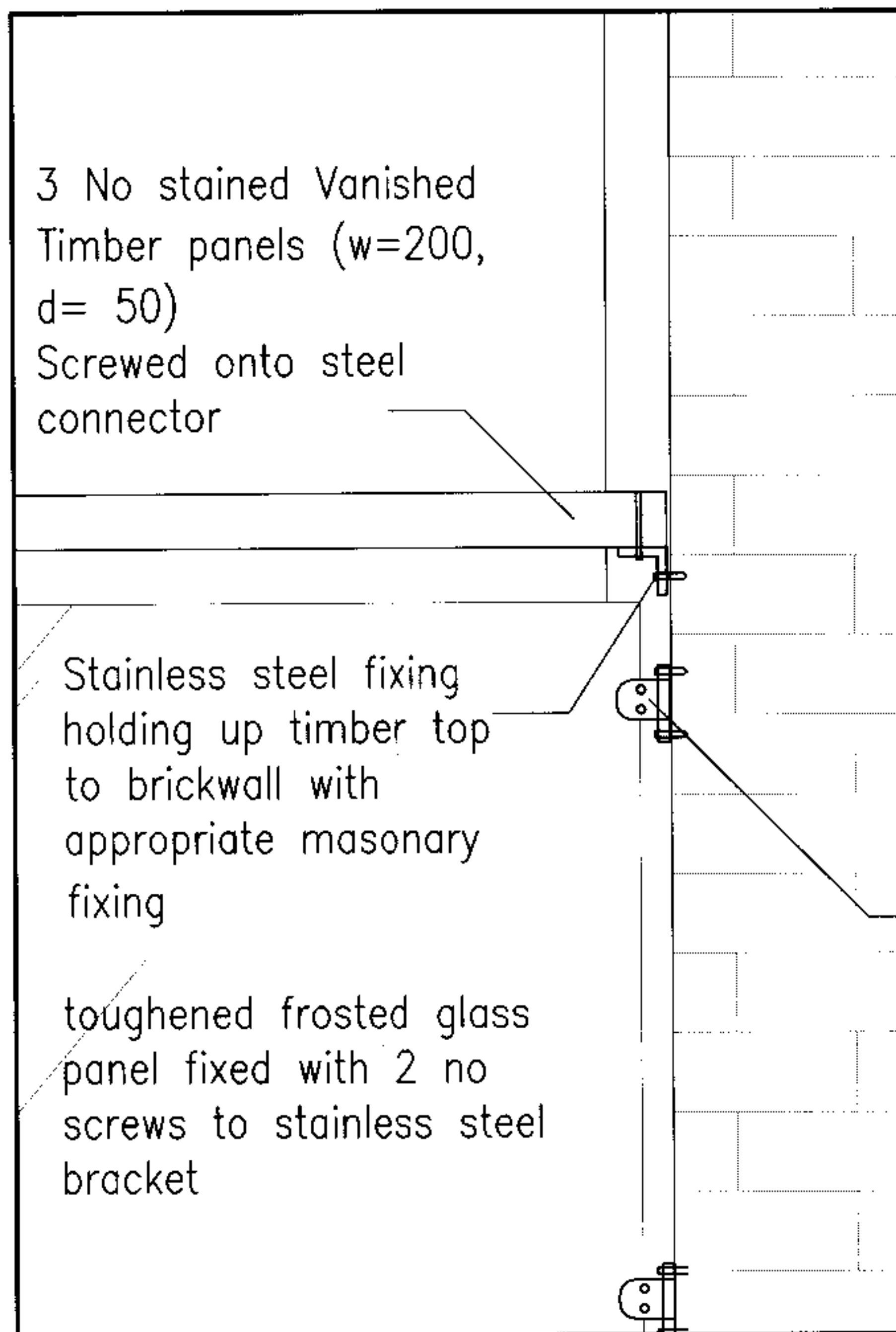
Detail 2 Scale 1:5
