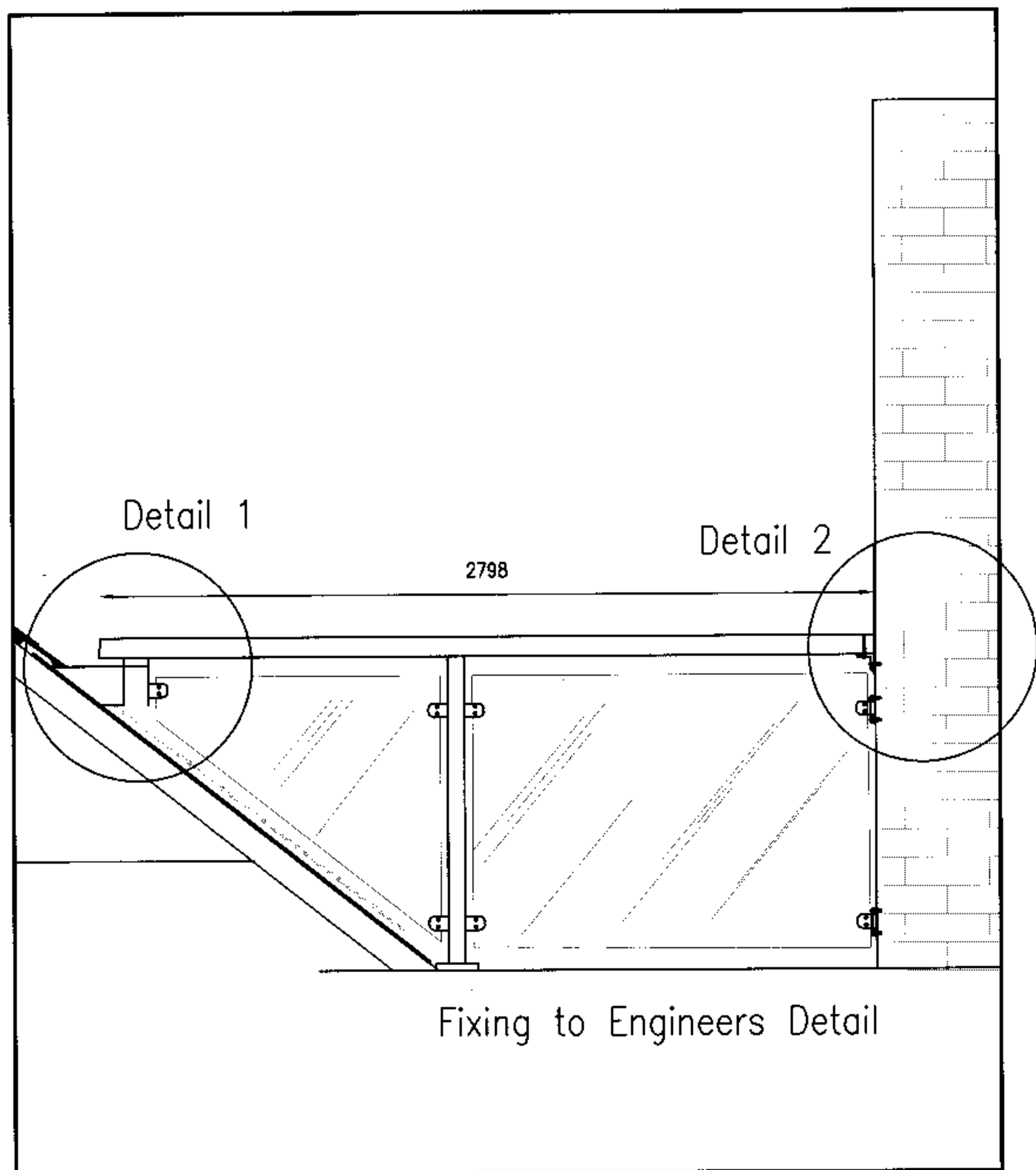
Elevation 1 Scale 1:25
