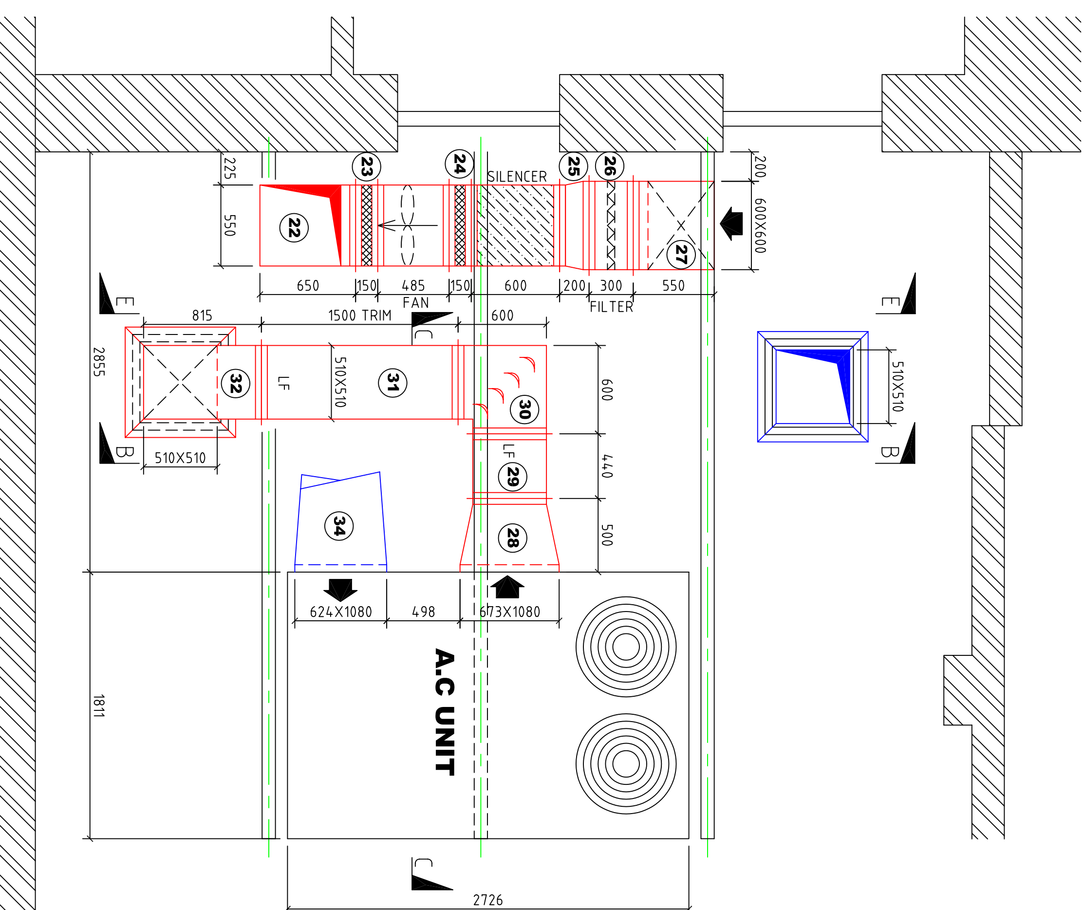
FLAT ROOF PLAN AT LOWER LEVEL
