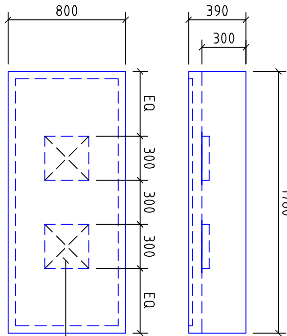
GROUND FLOOR STEAMER CONDENSE HOOD PLAN
