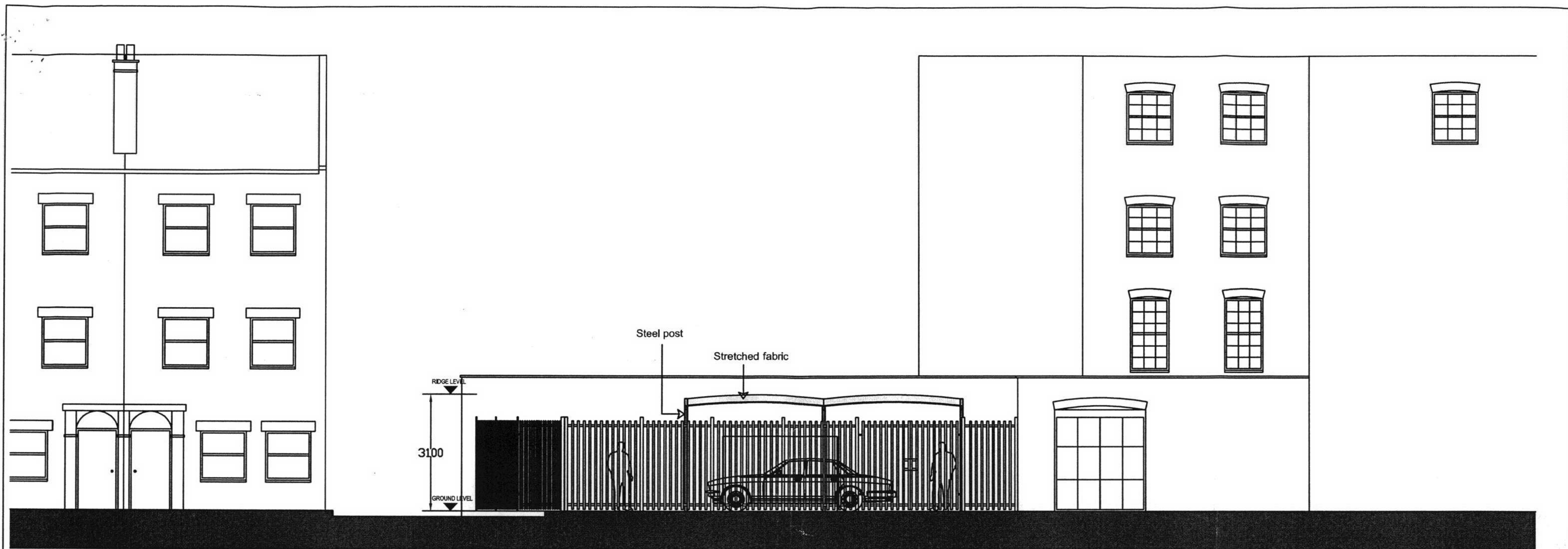
PROPOSED NORTH ELEVATION 1:100
