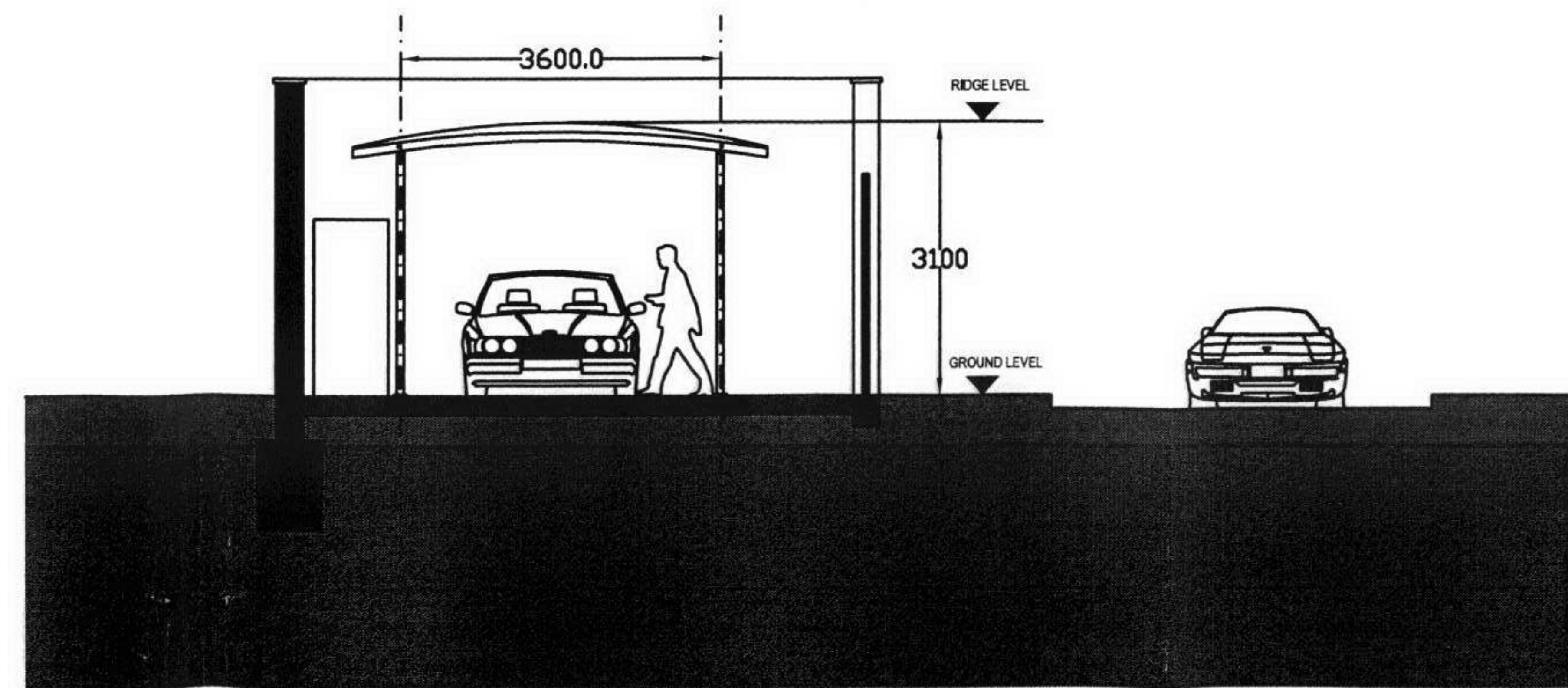
PROPOSED SECTION 1:100
