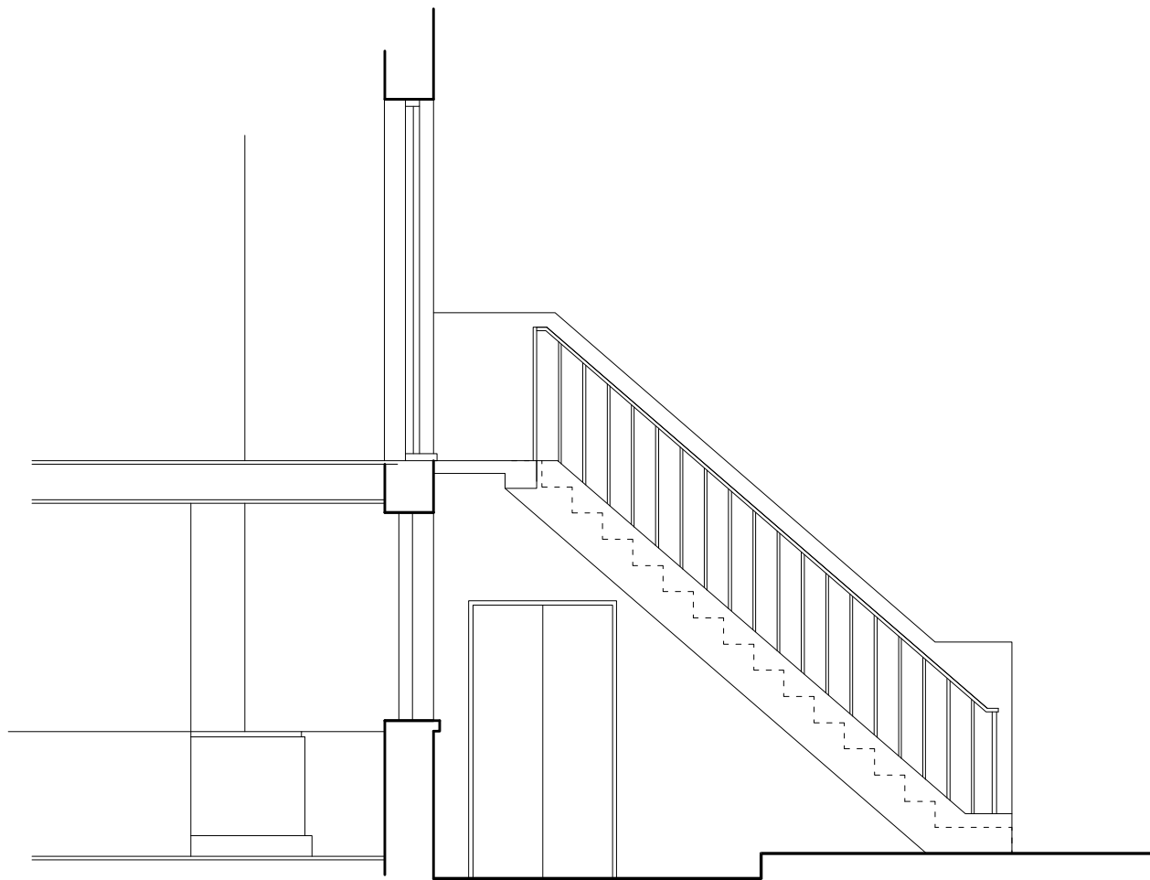
SECTION B-B
