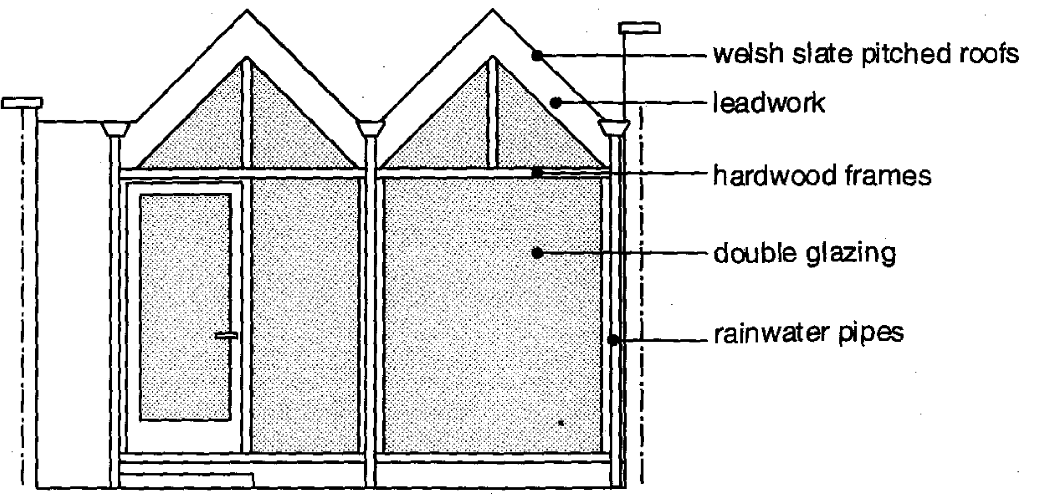
NEW EXTENSION ELEVATION 1:50
