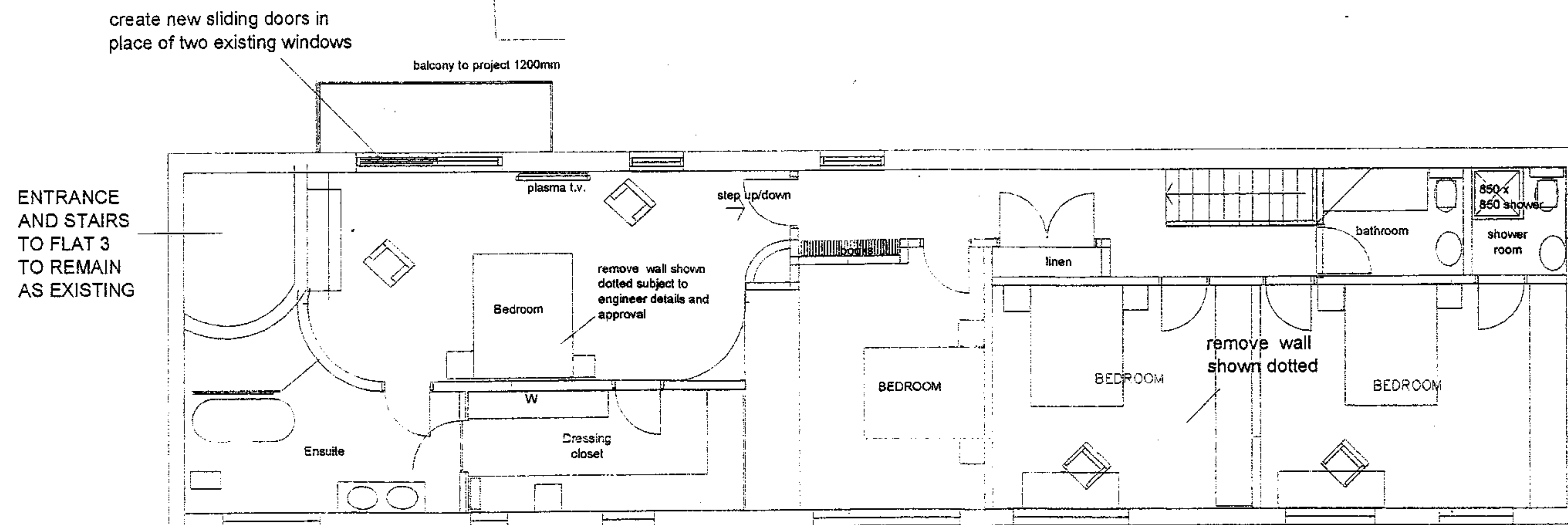
PROPOSED FIRST FLOOR LAYOUT showing preferred internal layout
