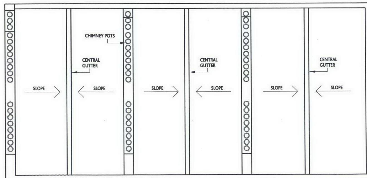
Roof Plan
