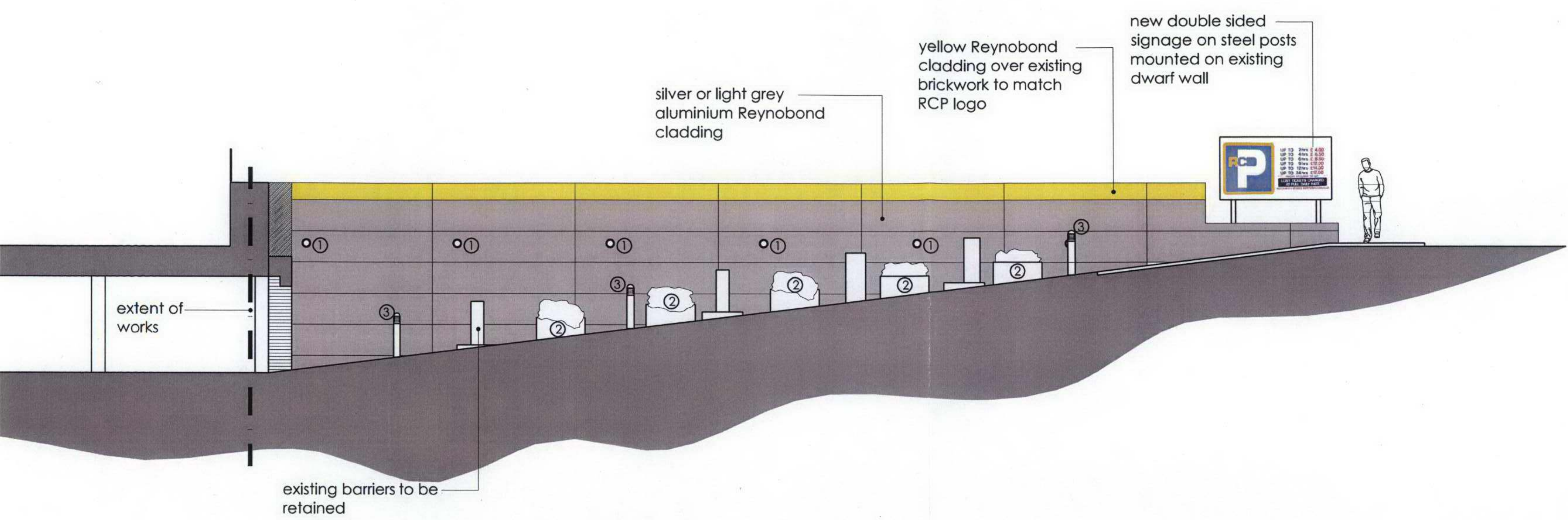
Section B-B - Option 1
