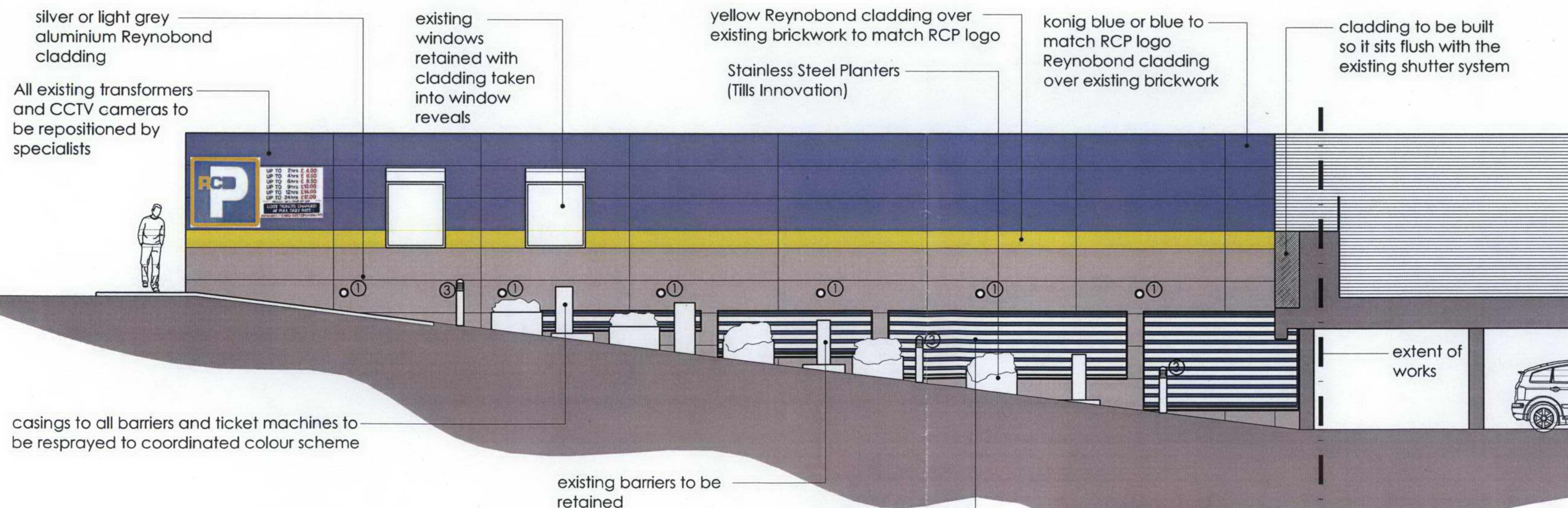
Section A-A - Option 1
