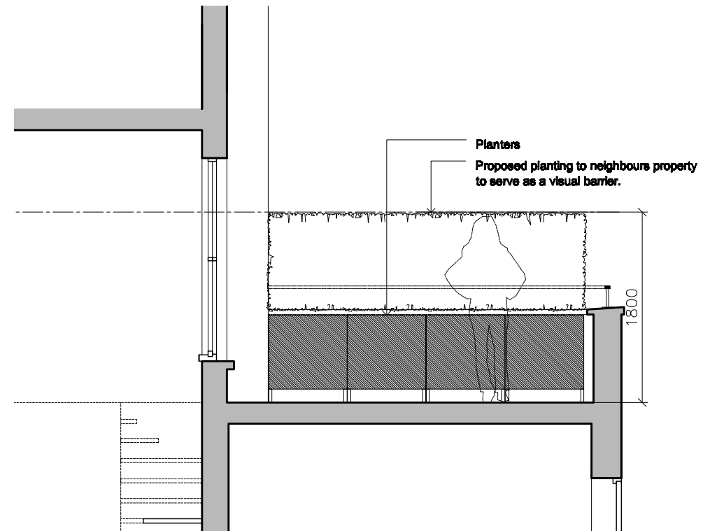
03 Section BB - Looking to no.7 Modbury Gardens 1:50
