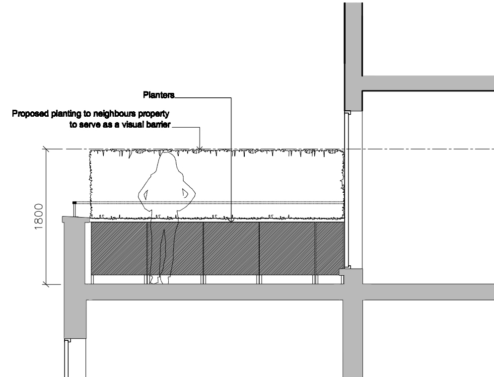
03 Section AA - Looking to no.6 Modbury Gardens 1:50
