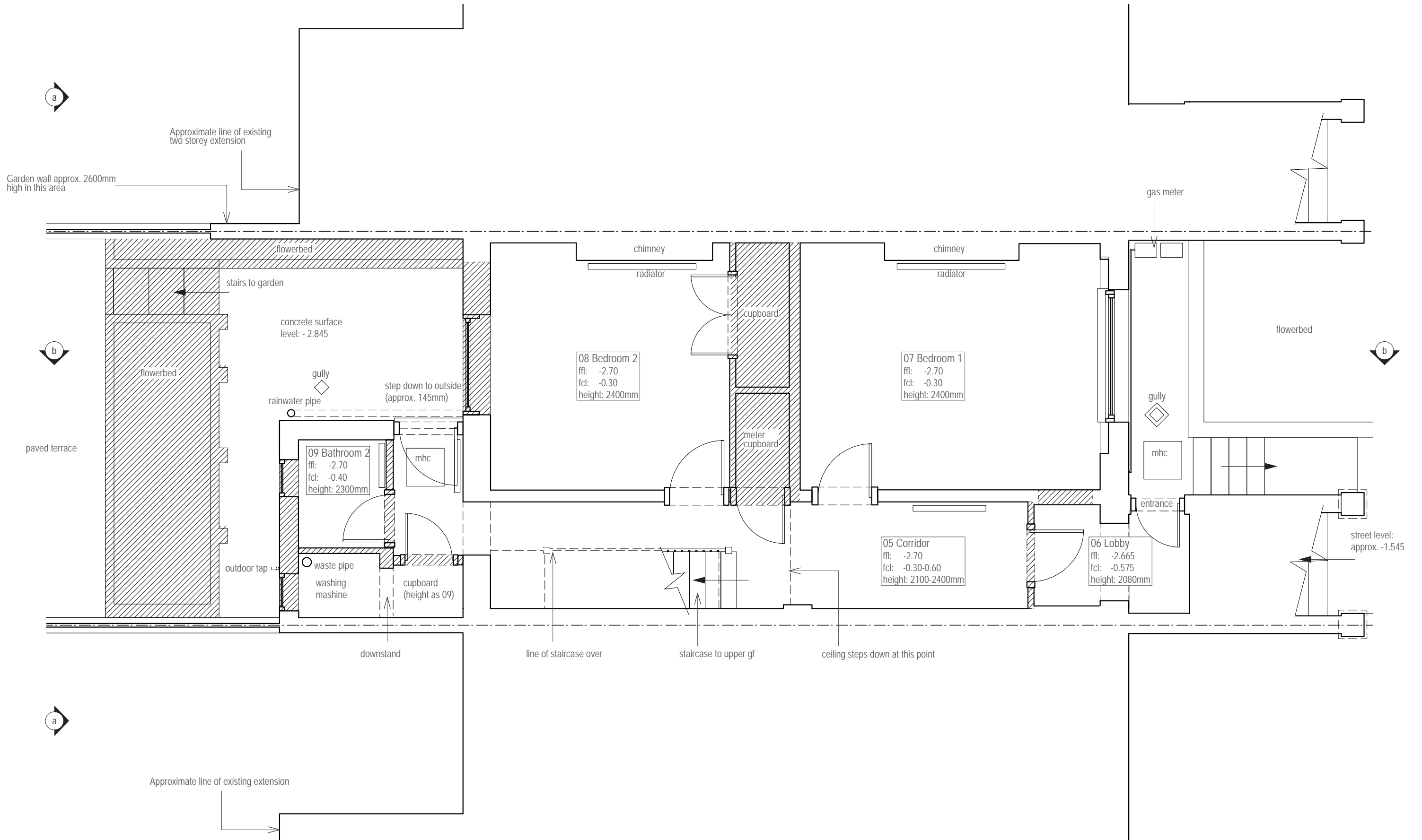
Lower ground floor plan as existing 1:50
