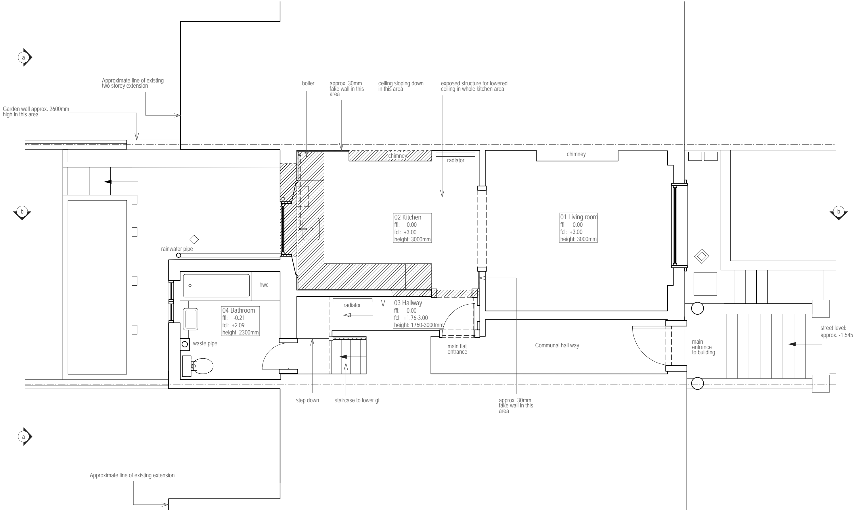
Upper ground floor plan as existing 1:50
