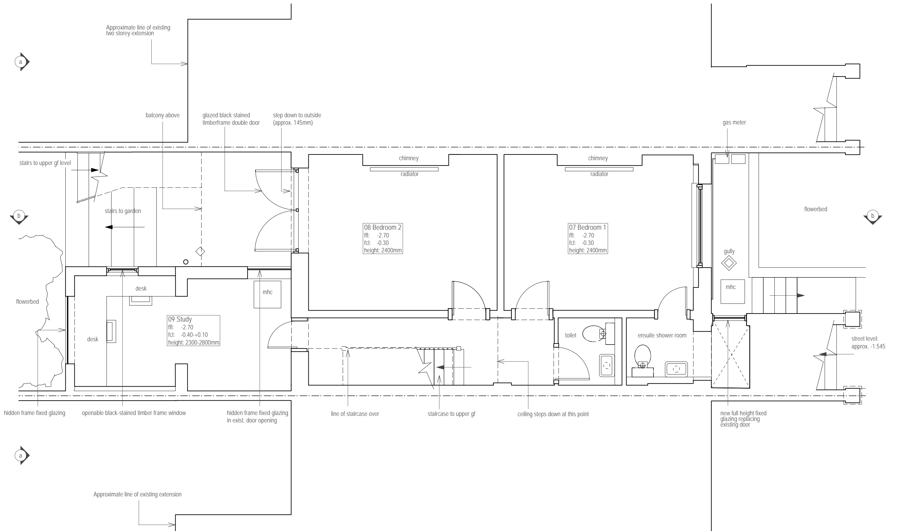
Lower ground floor plan as proposed 1:50
