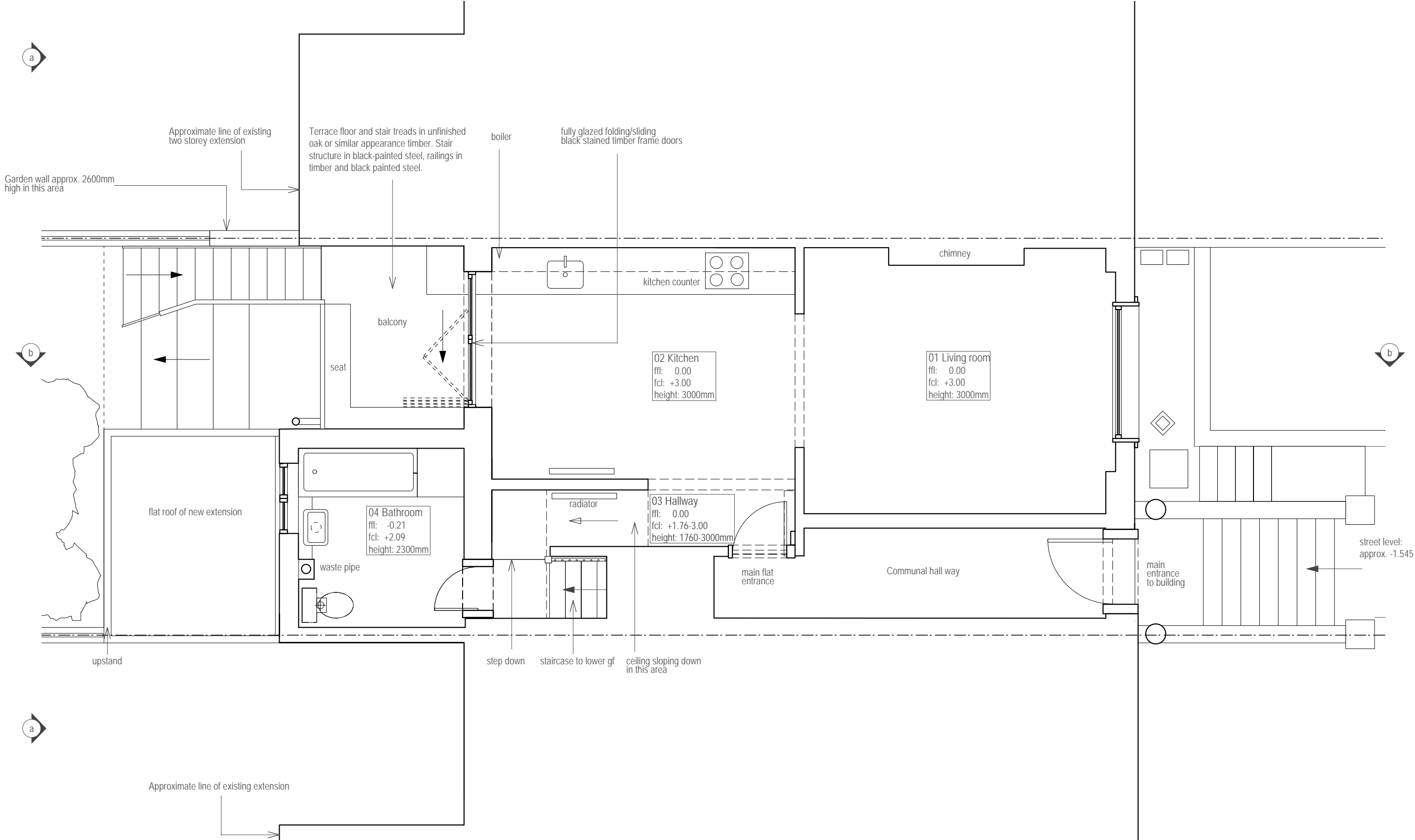
Upper ground floor plan as proposed 1:50
