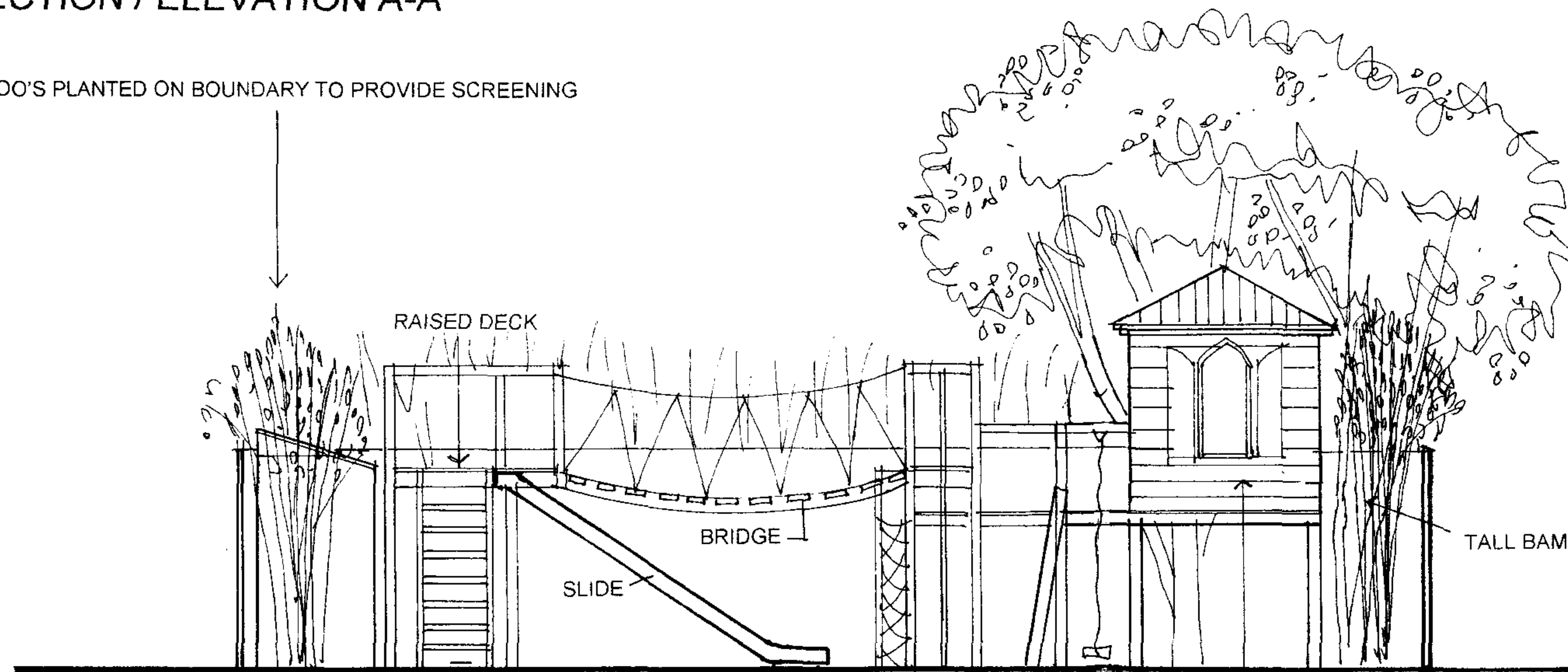
SECTION / ELEVATION A-A
