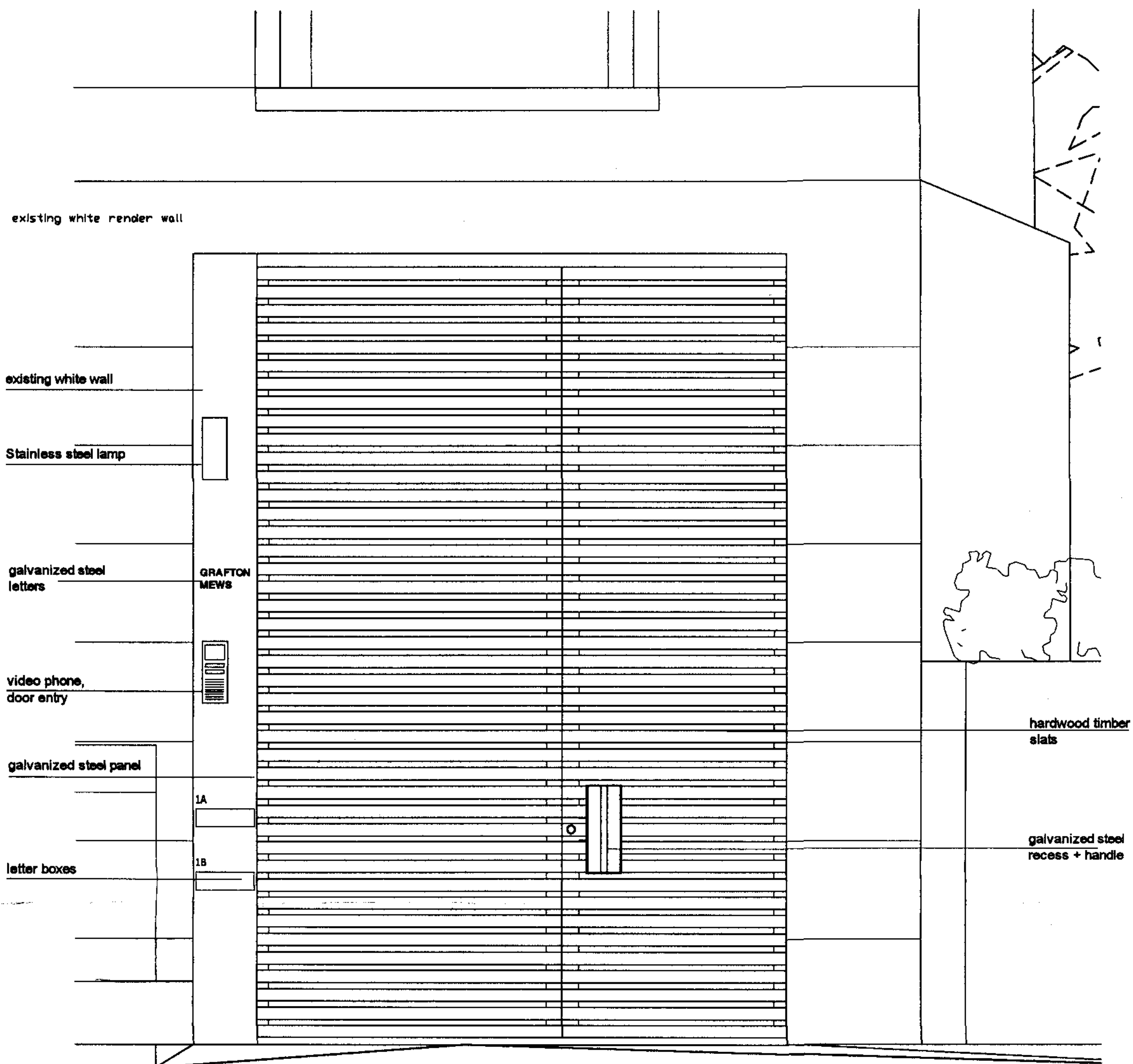
GATE ELVATION AT 1:20
