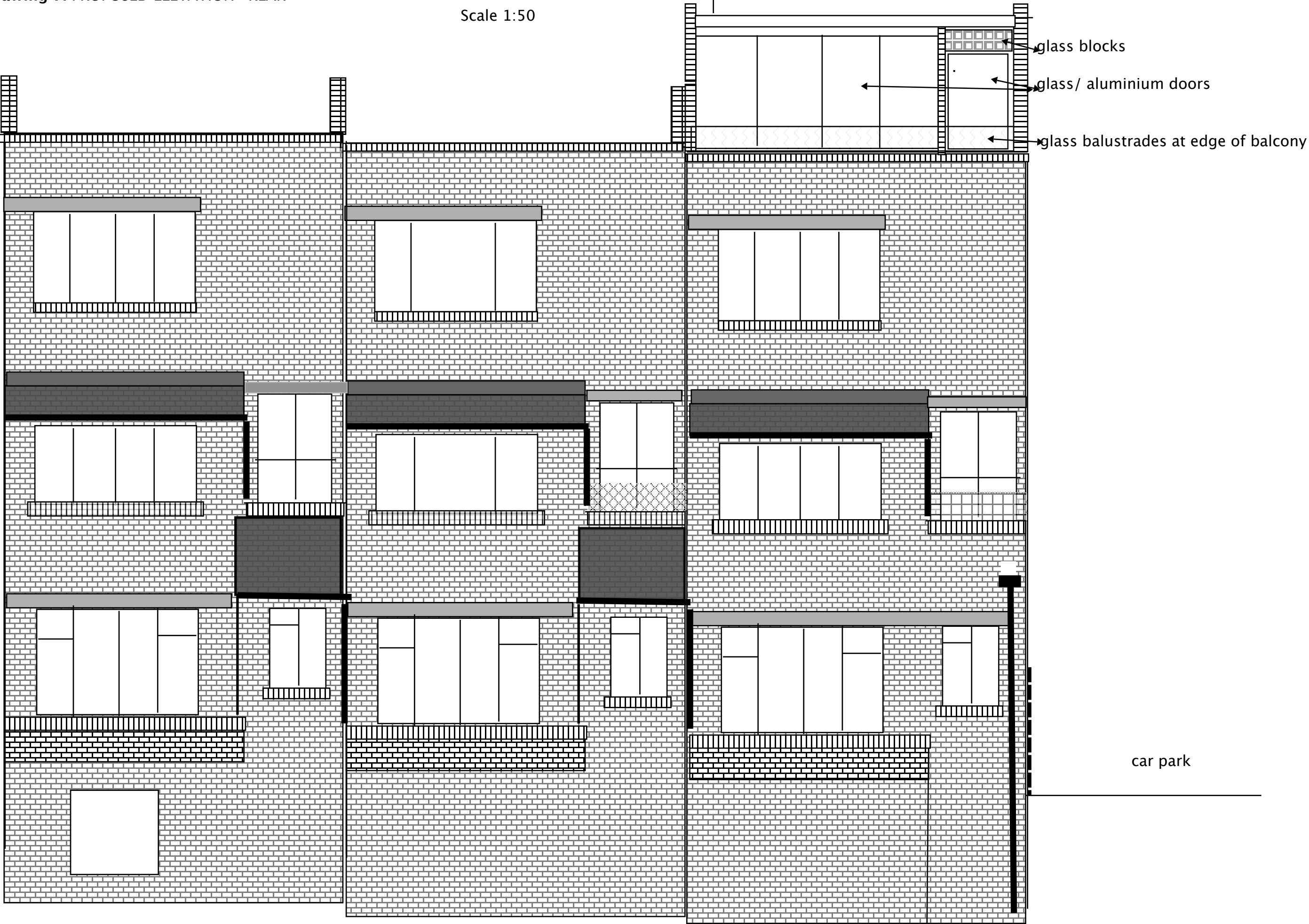
Drawing 7: PROPOSED ELEVATION– REAR
