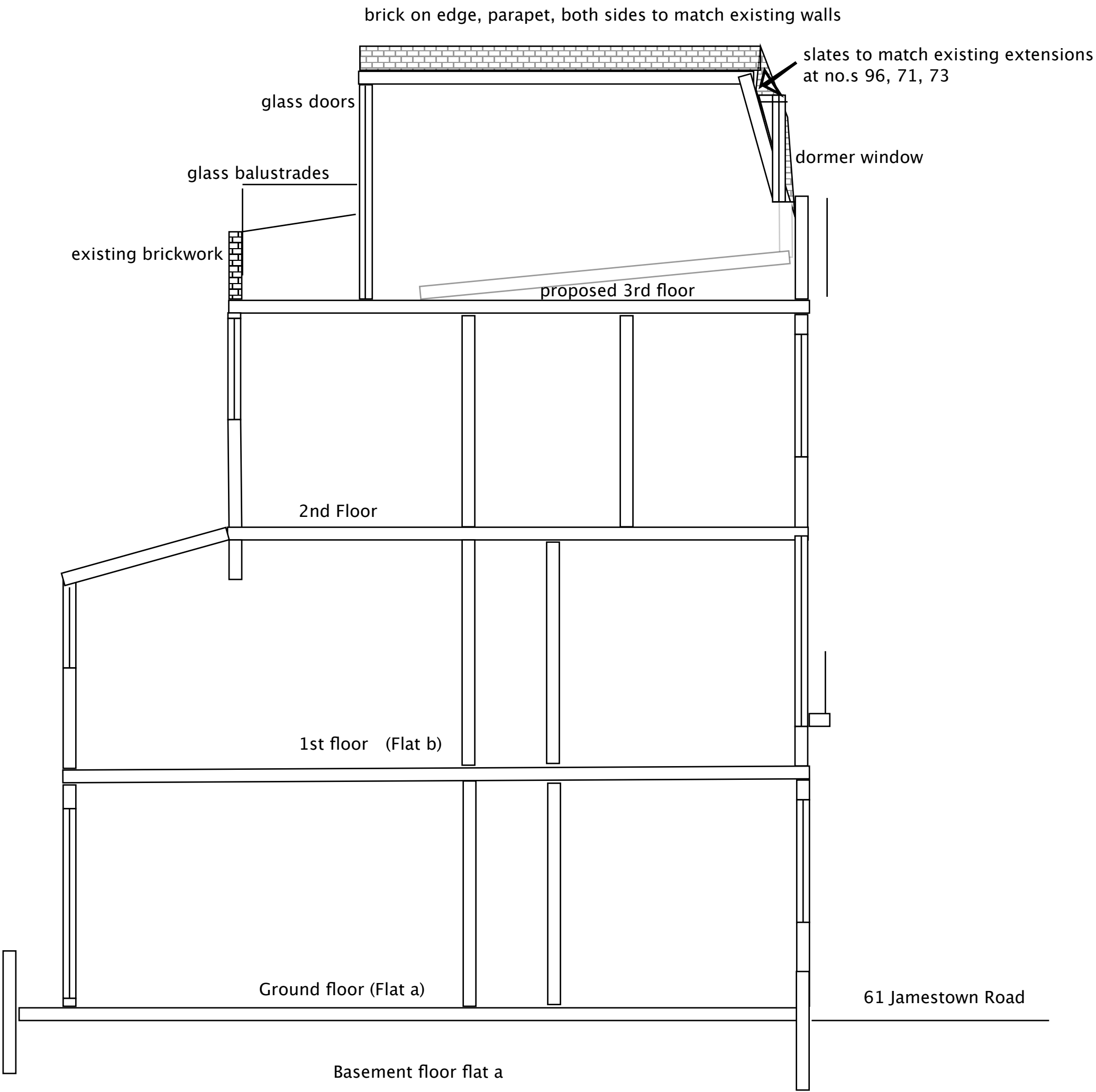
Drawing 9: Proposed Section
