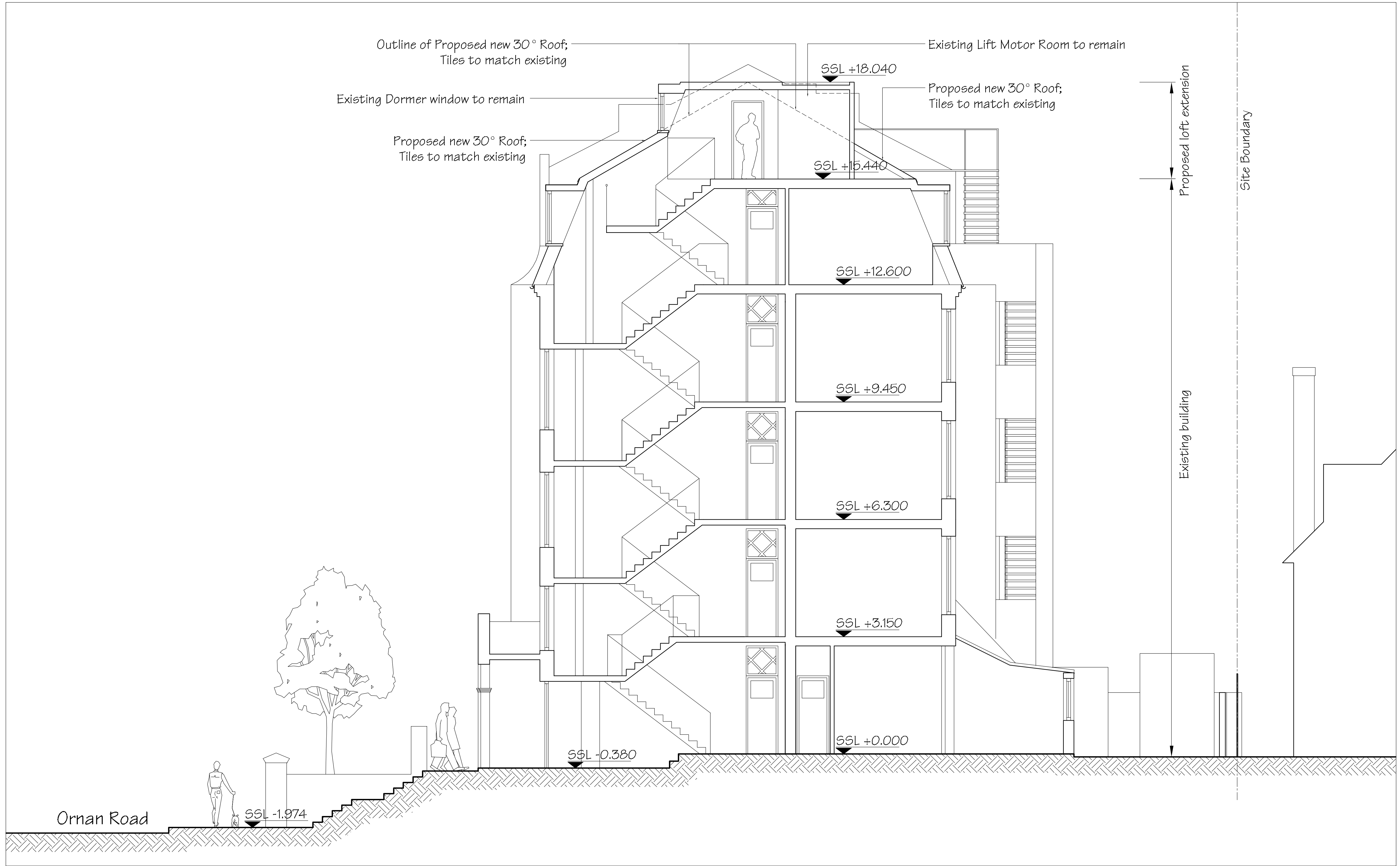
Cross Section A-A as Proposed 2 Ornan Court, Ornan Road, London NW3 4PT
