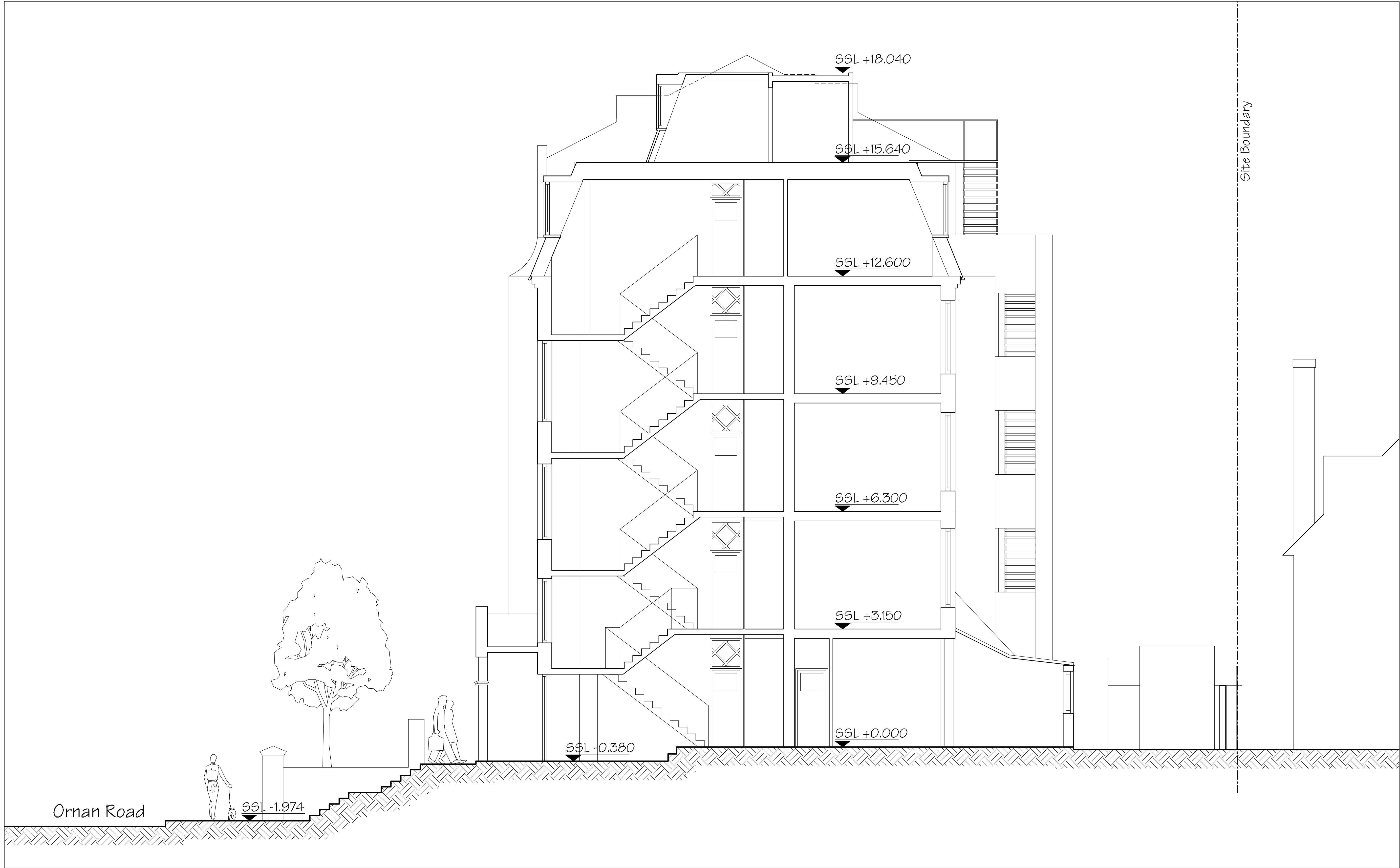
Cross Section A-A as Existing 2 Ornan Court, Ornan Road, London NW3 4PT
