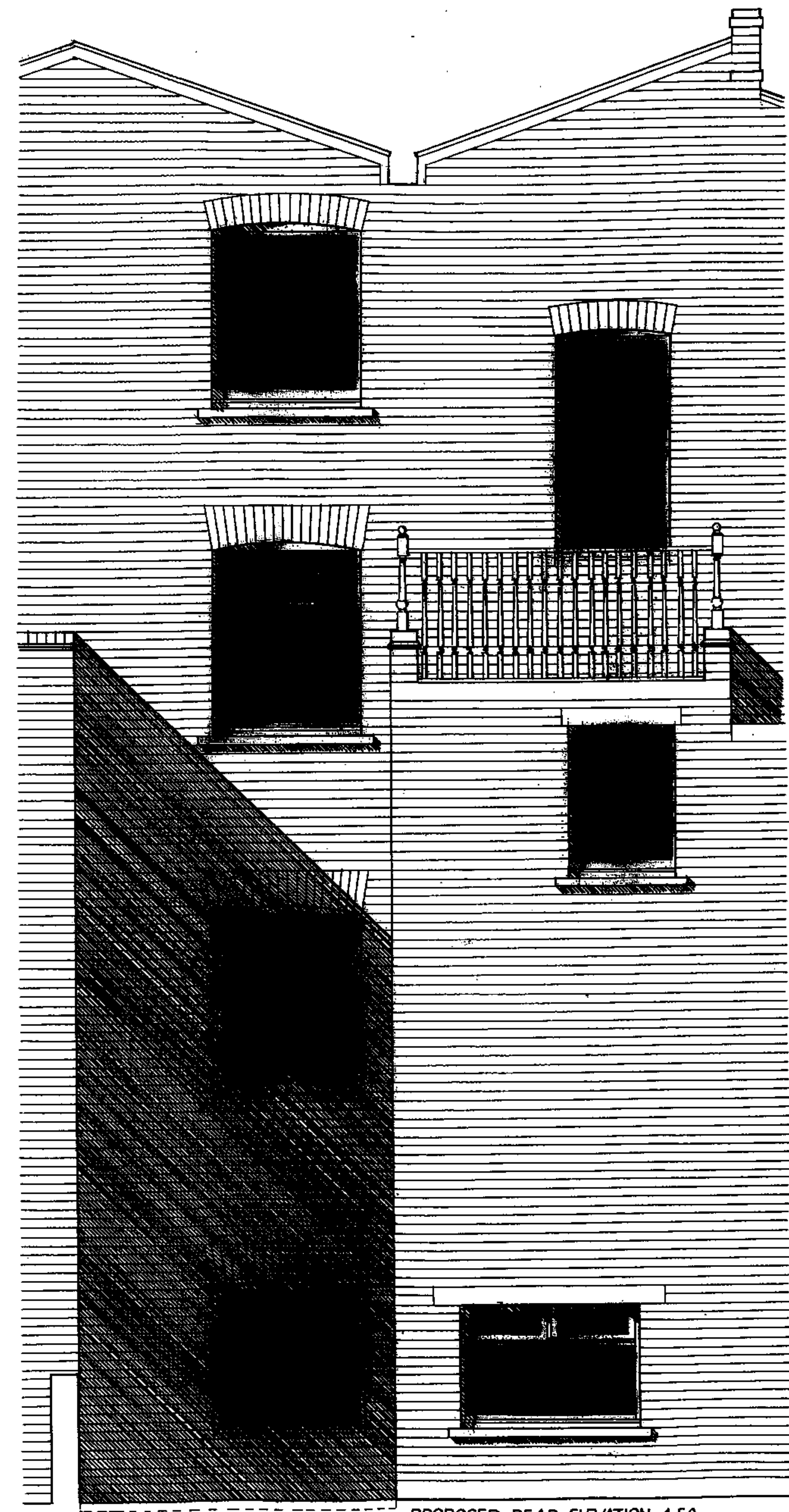
PROPOSED REAR ELEVATION 1:50
