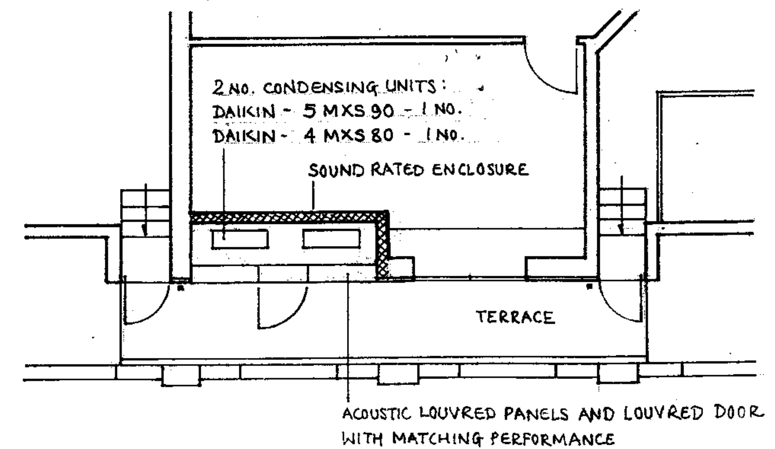
PLAN AT 2 ND FLOOR ROOF TERRACE
