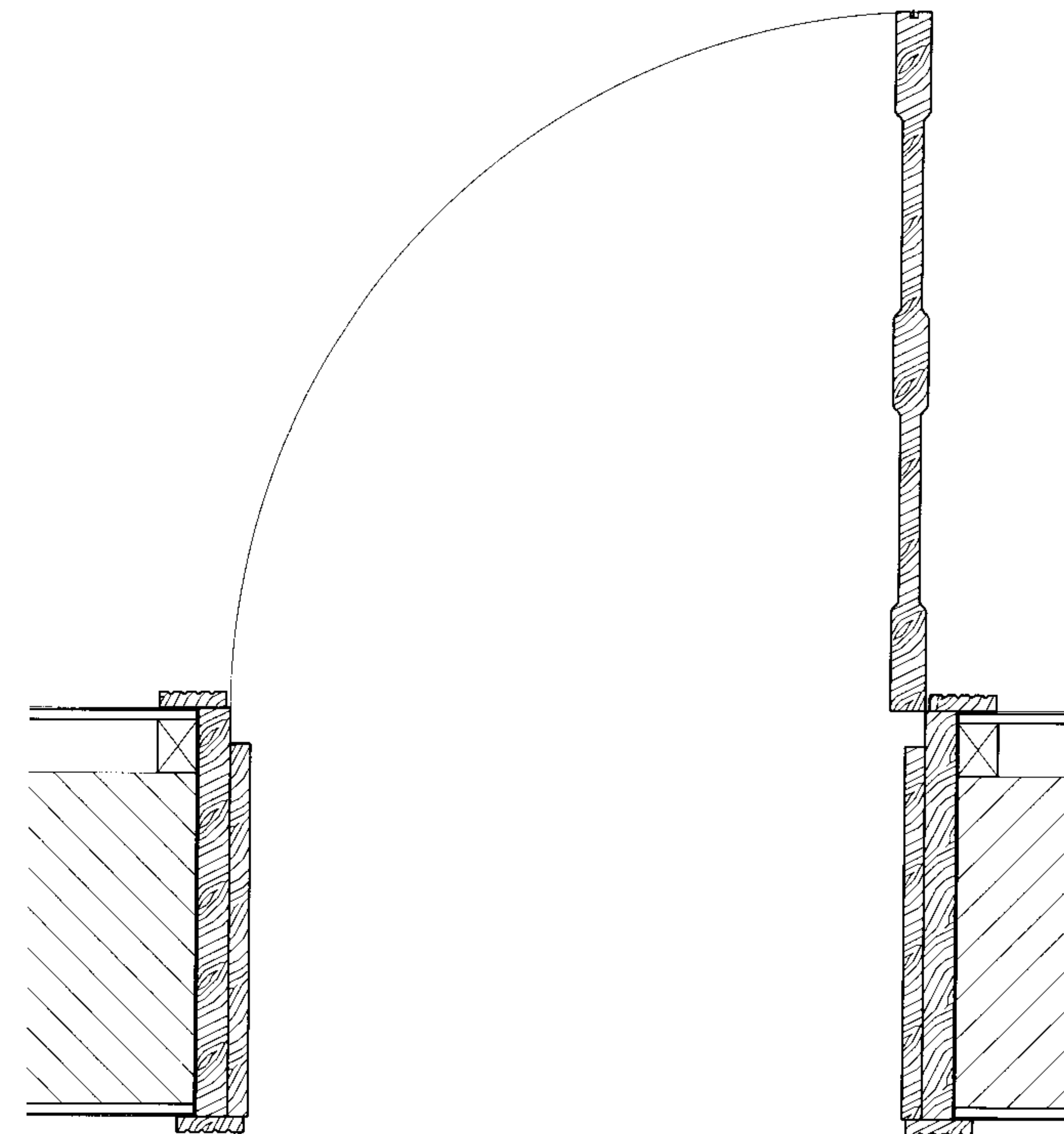
D03.01 FD30 DOOR PLAN SCALE 1:10 PANELING AND ARCHITRAVES TO MATCH EXISTING
