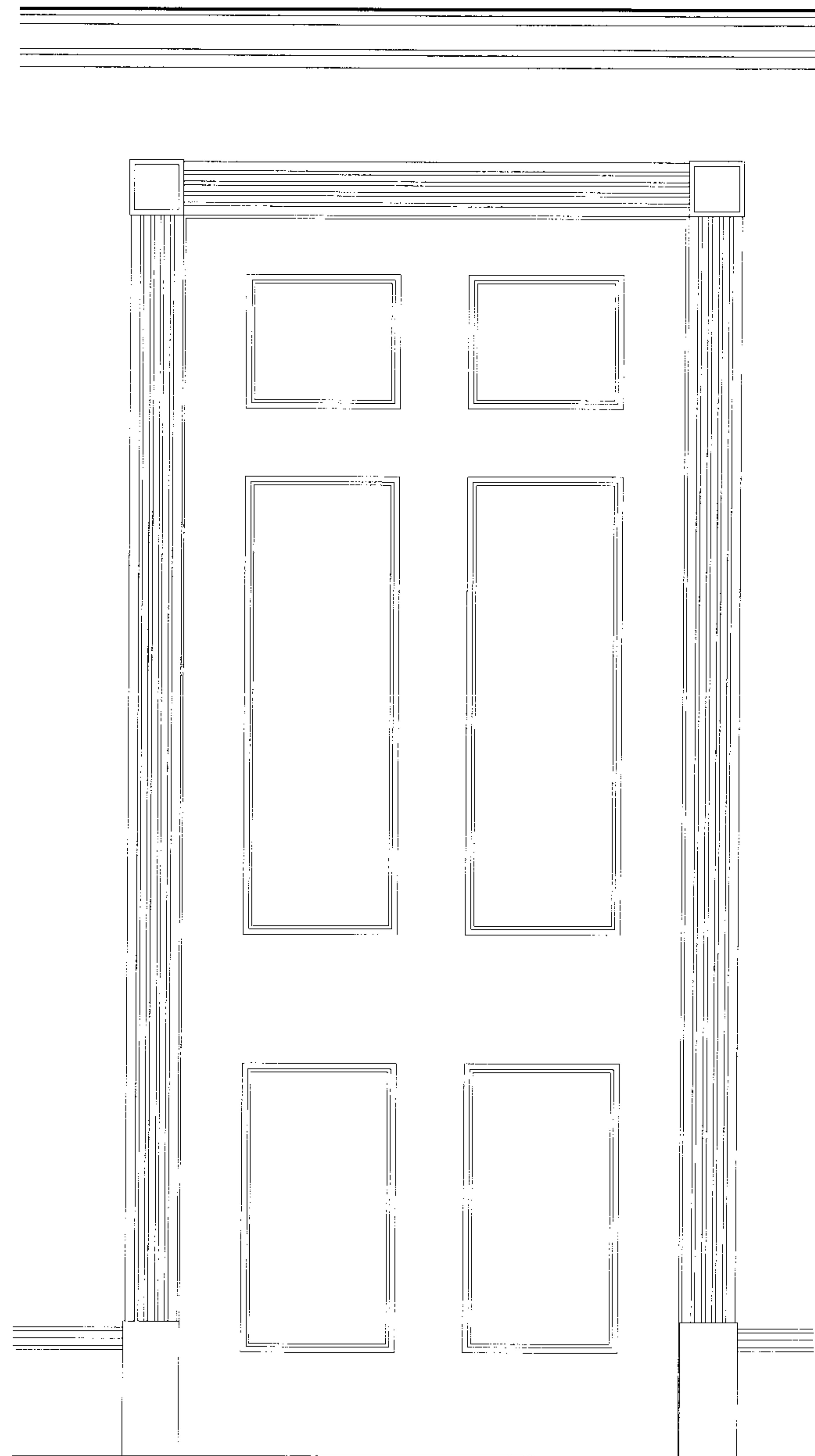
D03.01 FD30 DOOR ELEVATION SCALE 1:10 PANELING AND ARCHITRAVES TO MATCH EXISTING
