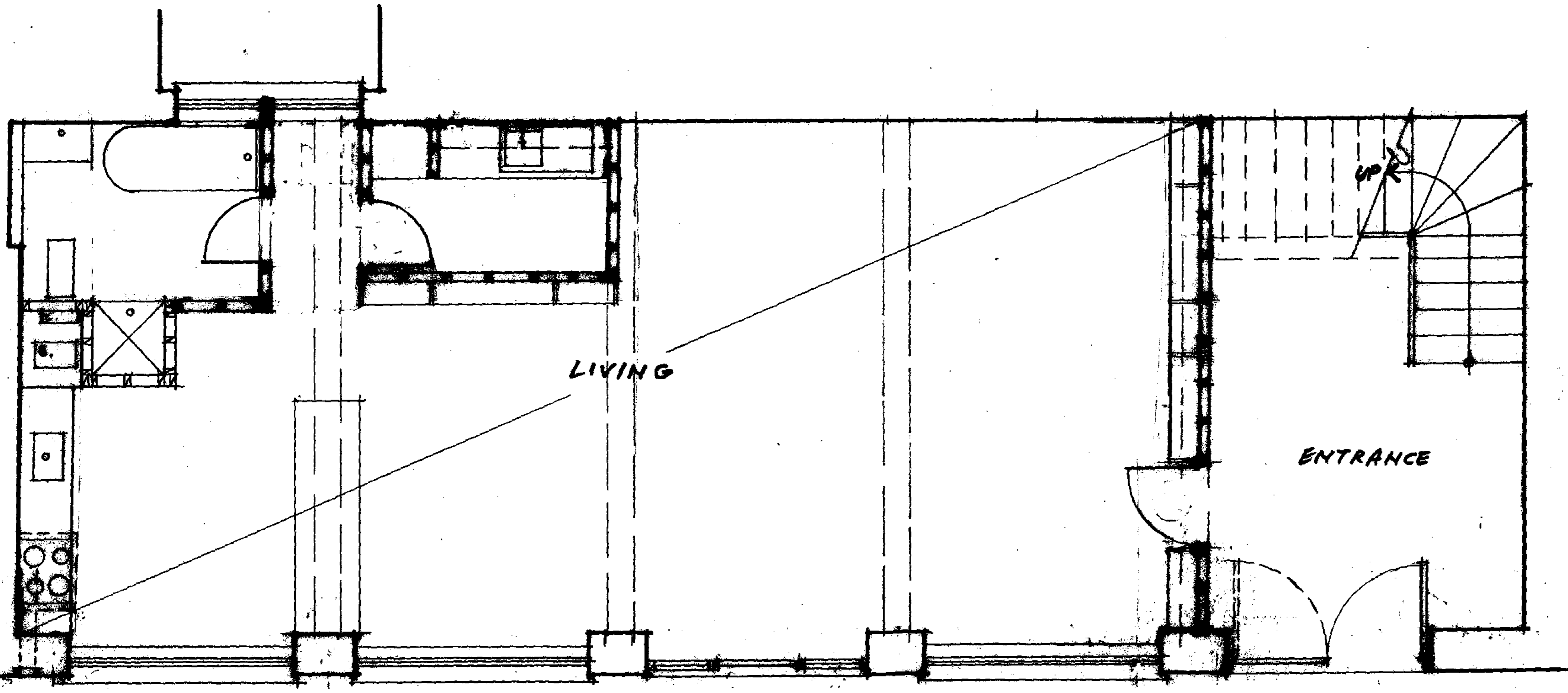
PROPOSED GROUND FLOOR.
