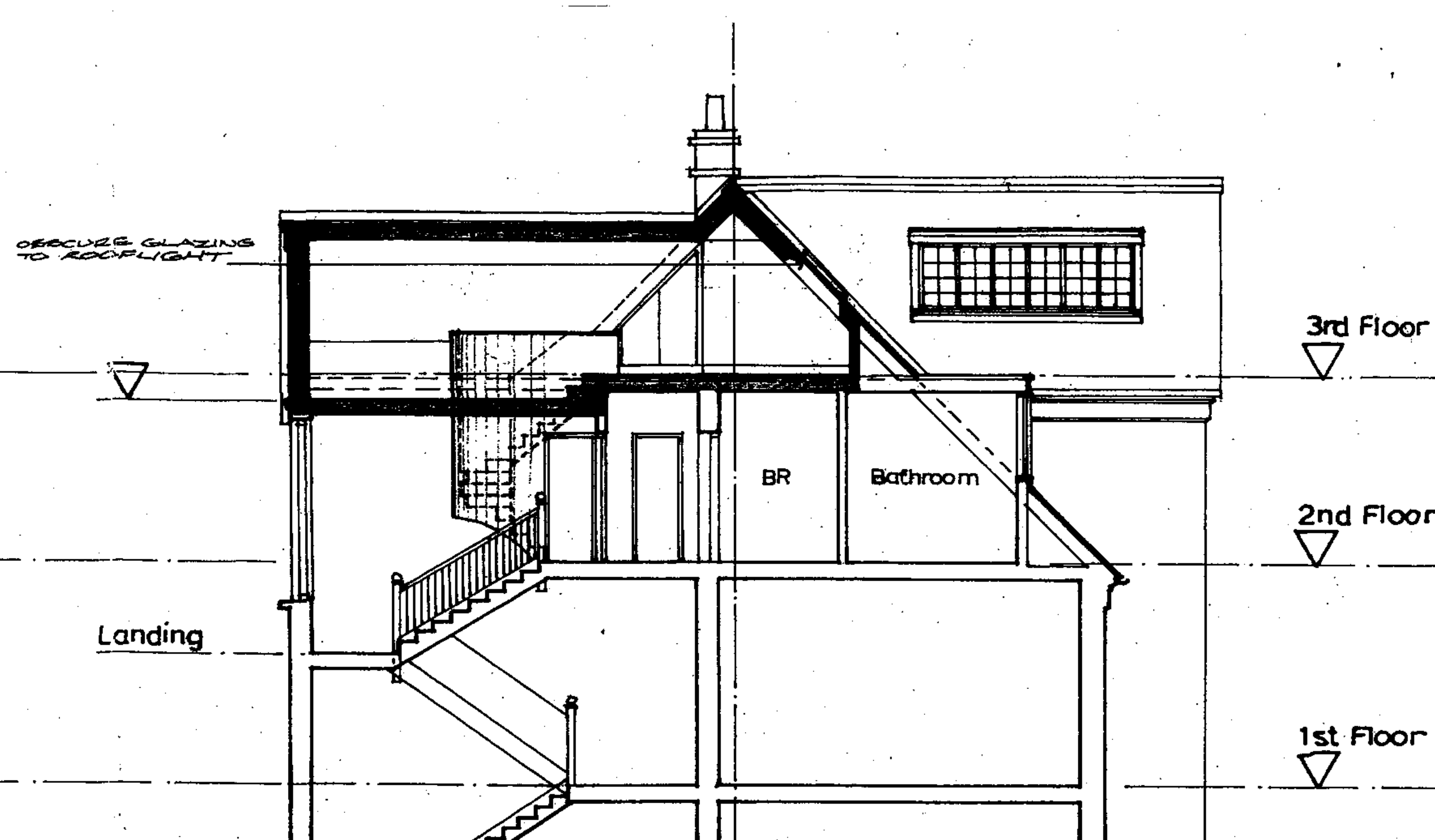
B-B Proposed
