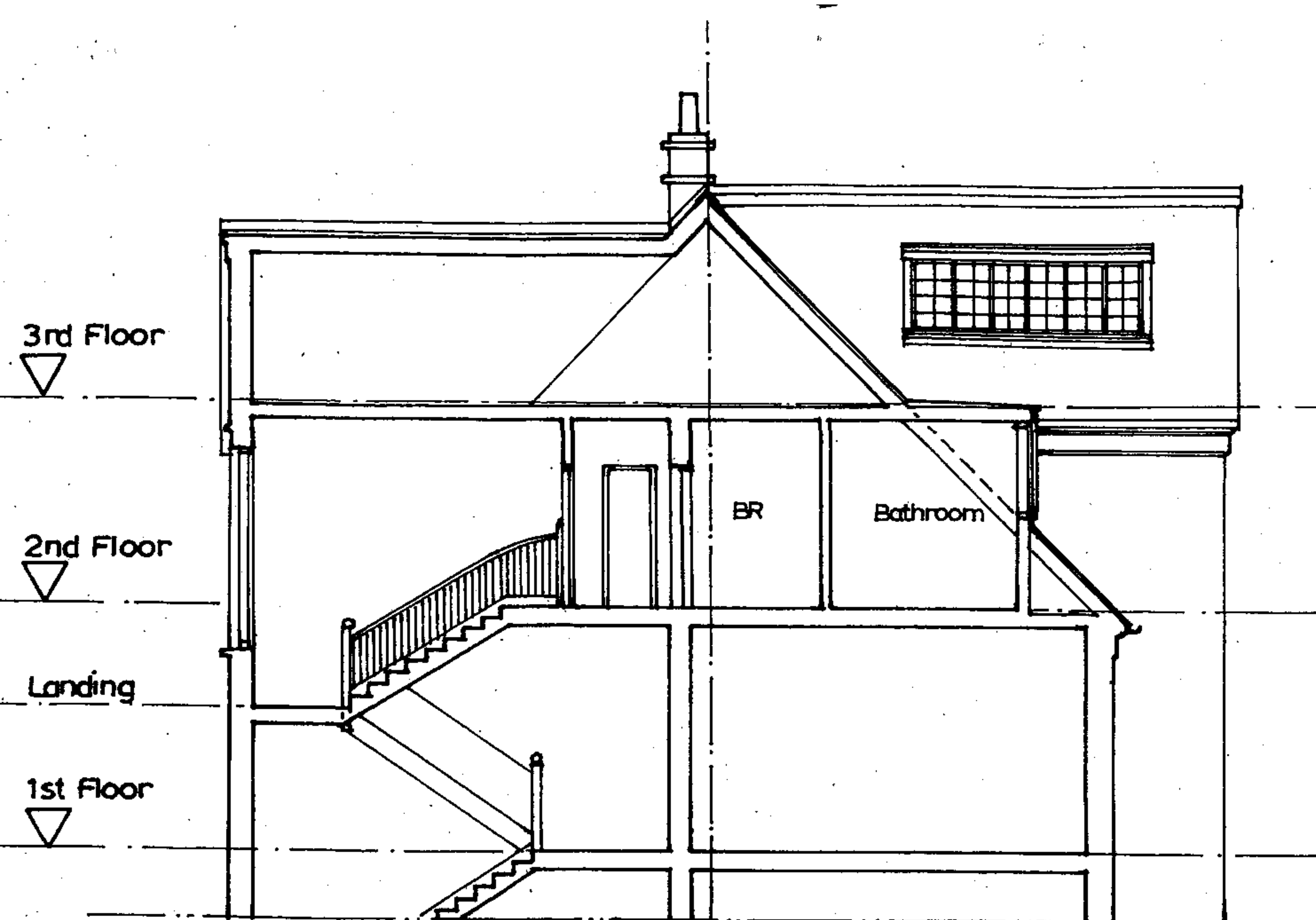
A-A Existing.
