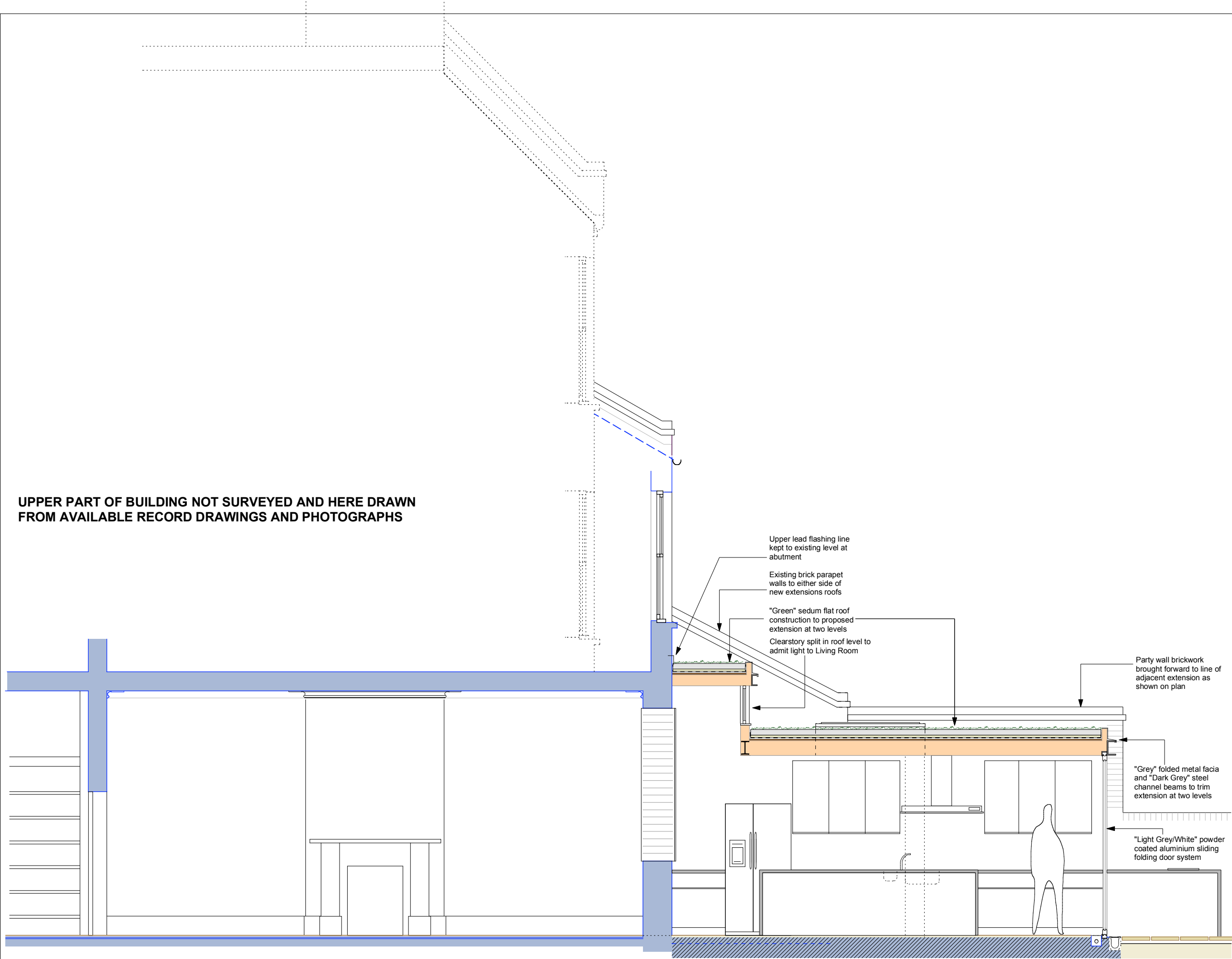
Section A-A : Part Ground Floor Rear : Front to Back Section : Proposed Scale 1:50
