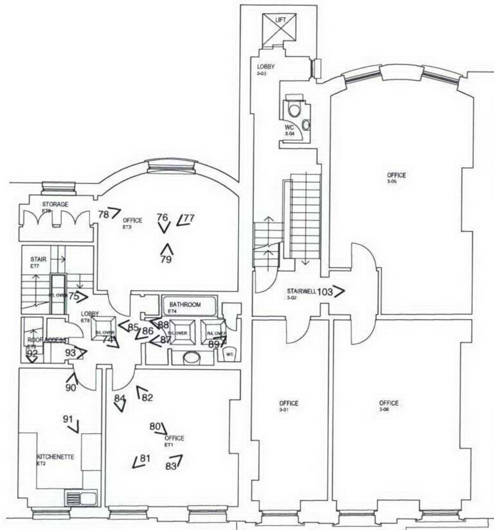
THIRD FLOOR
