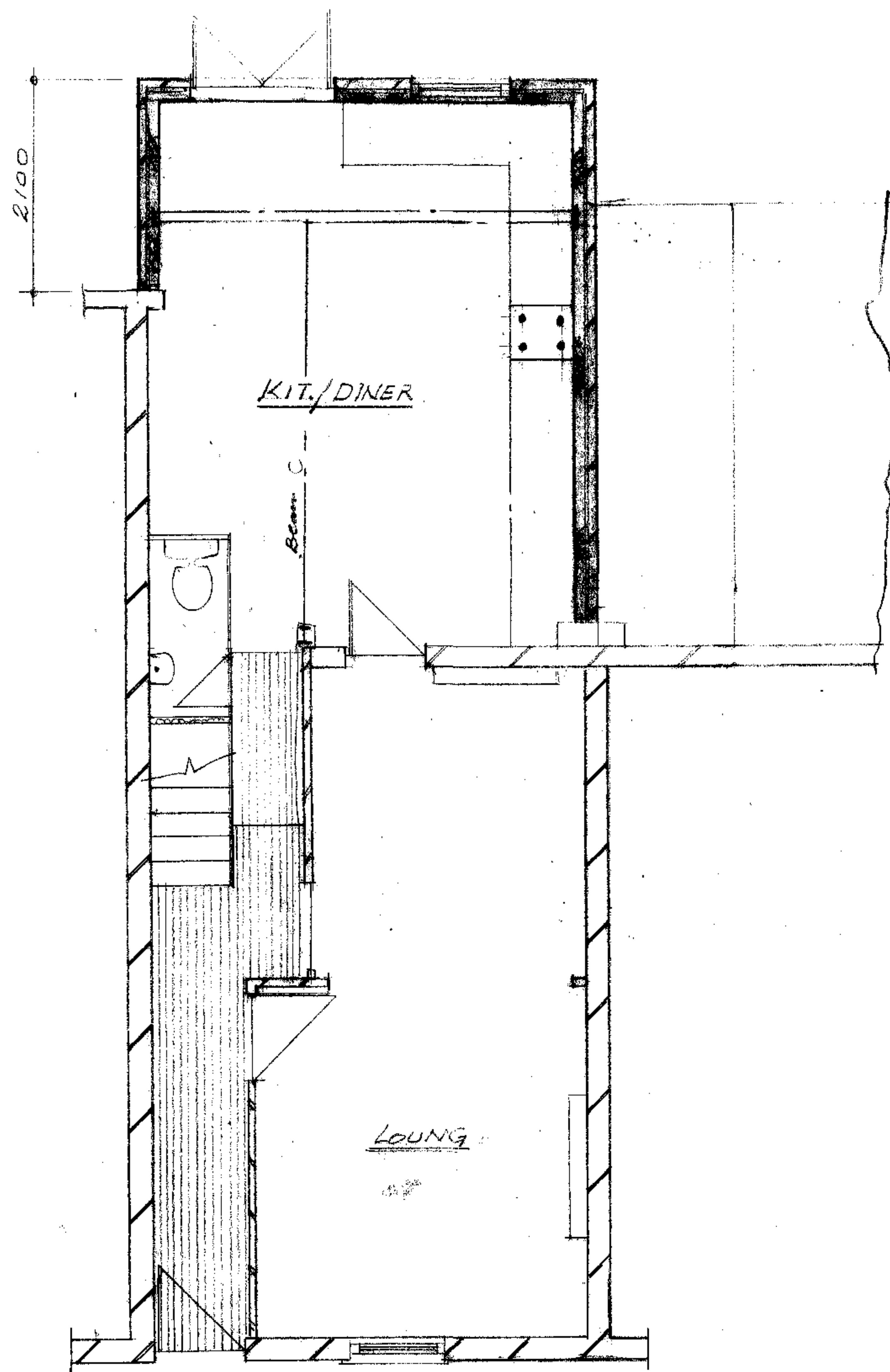
PROP. G.F. PLAN
