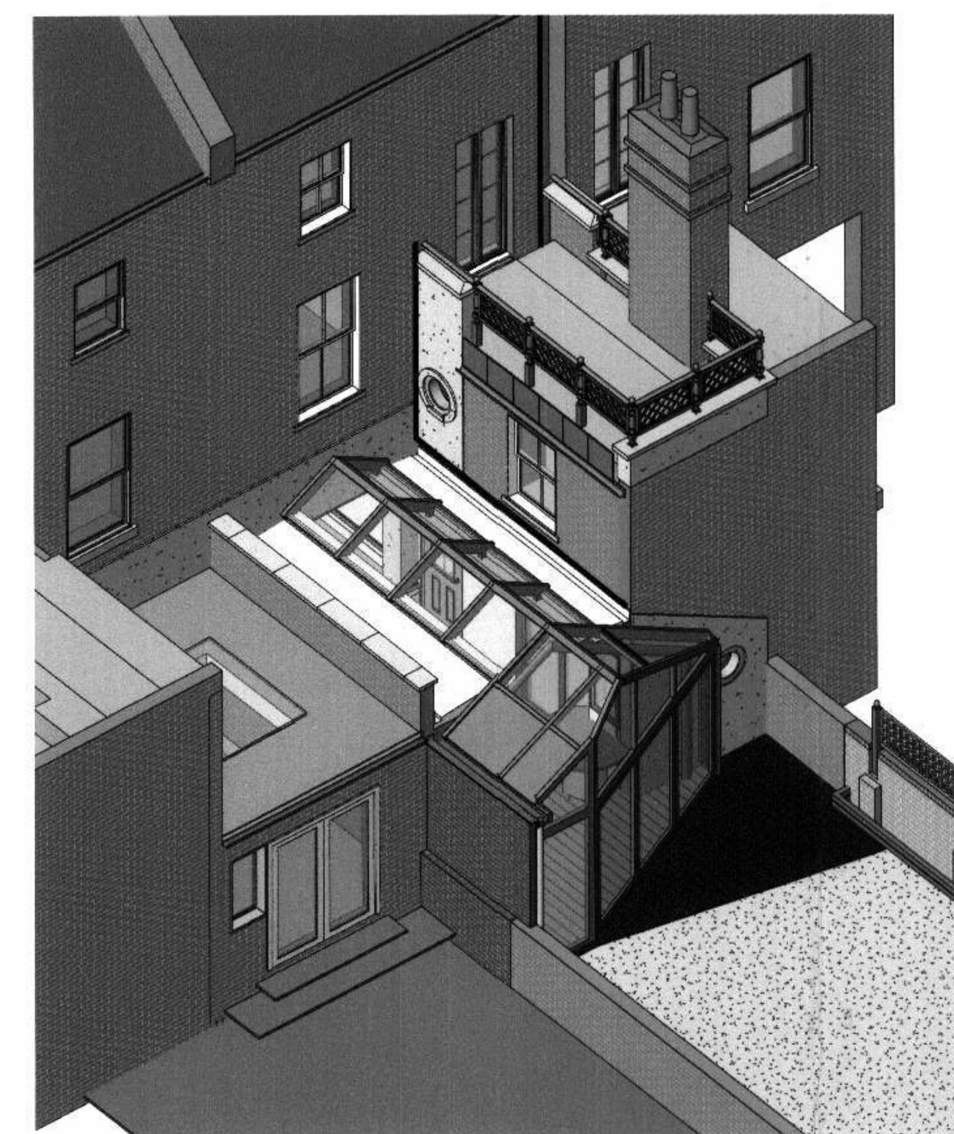
3 Rear Isometric View as Proposed
