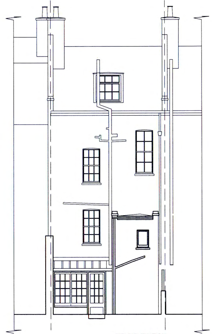
REAR ELEVATION
