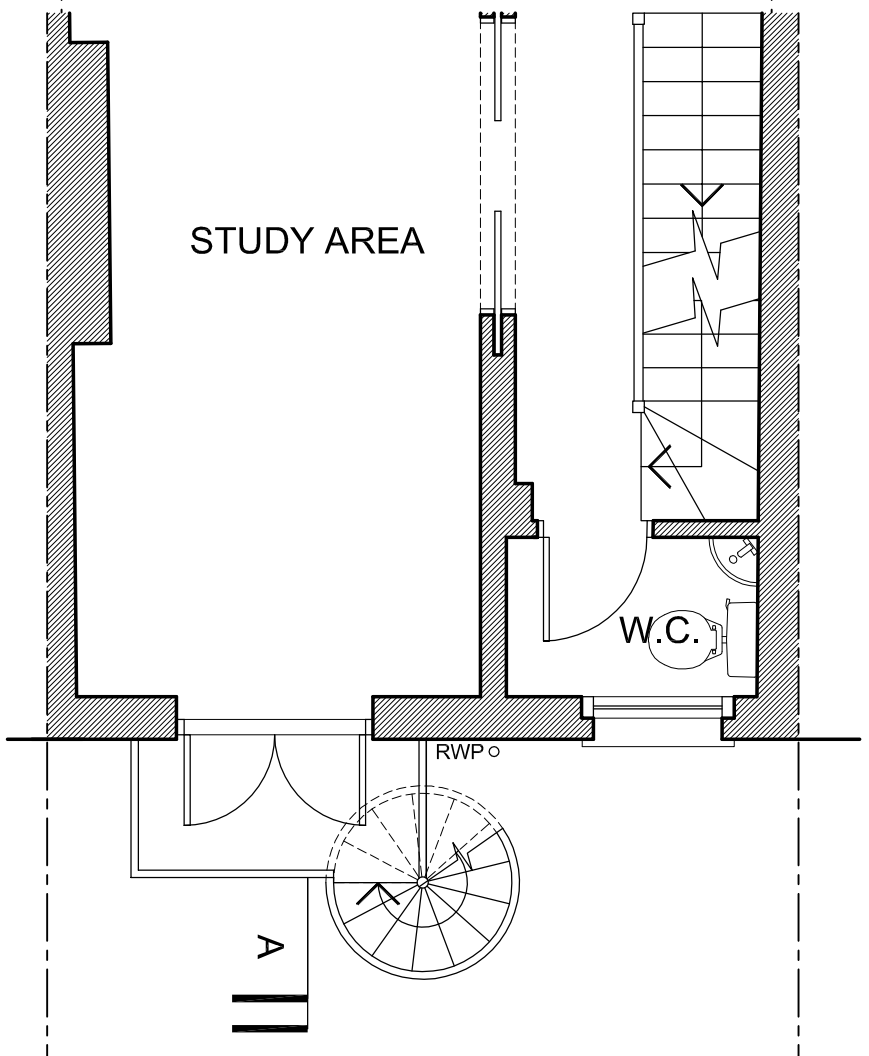
Part Ground Floor Plan
