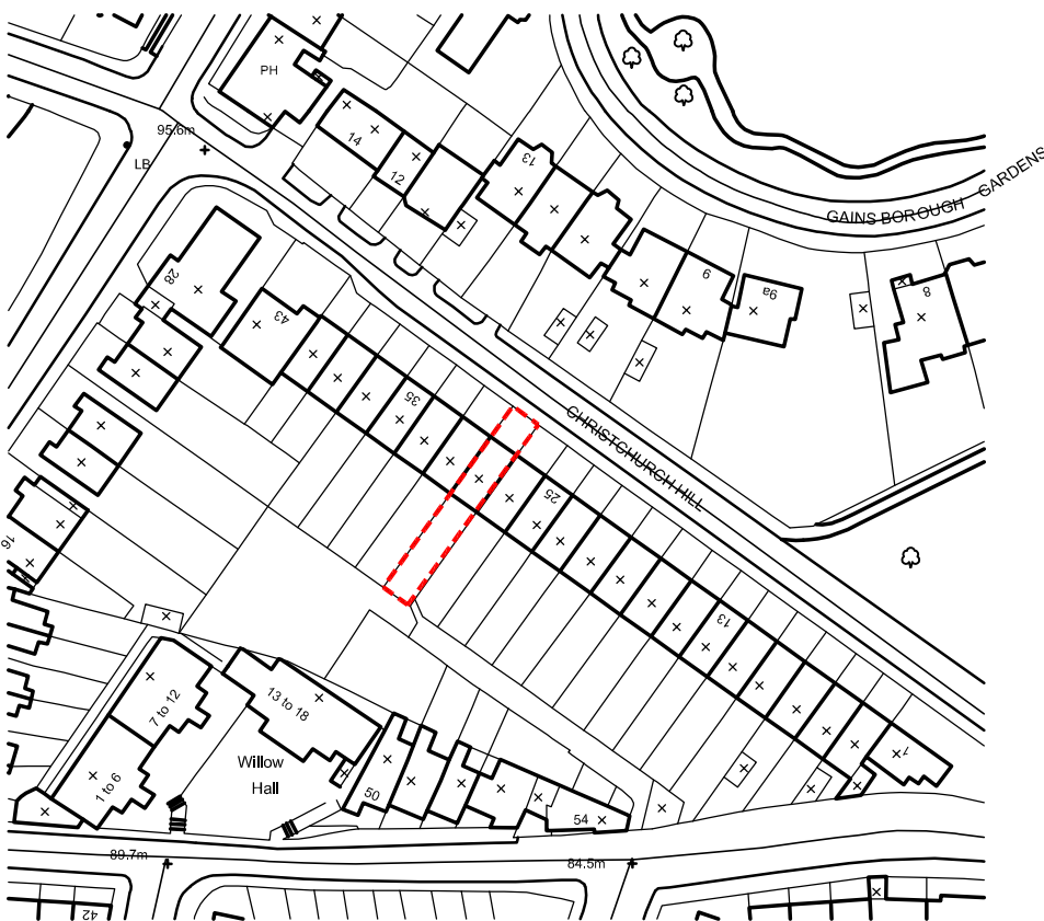
SITE PLAN @ 1/1250
