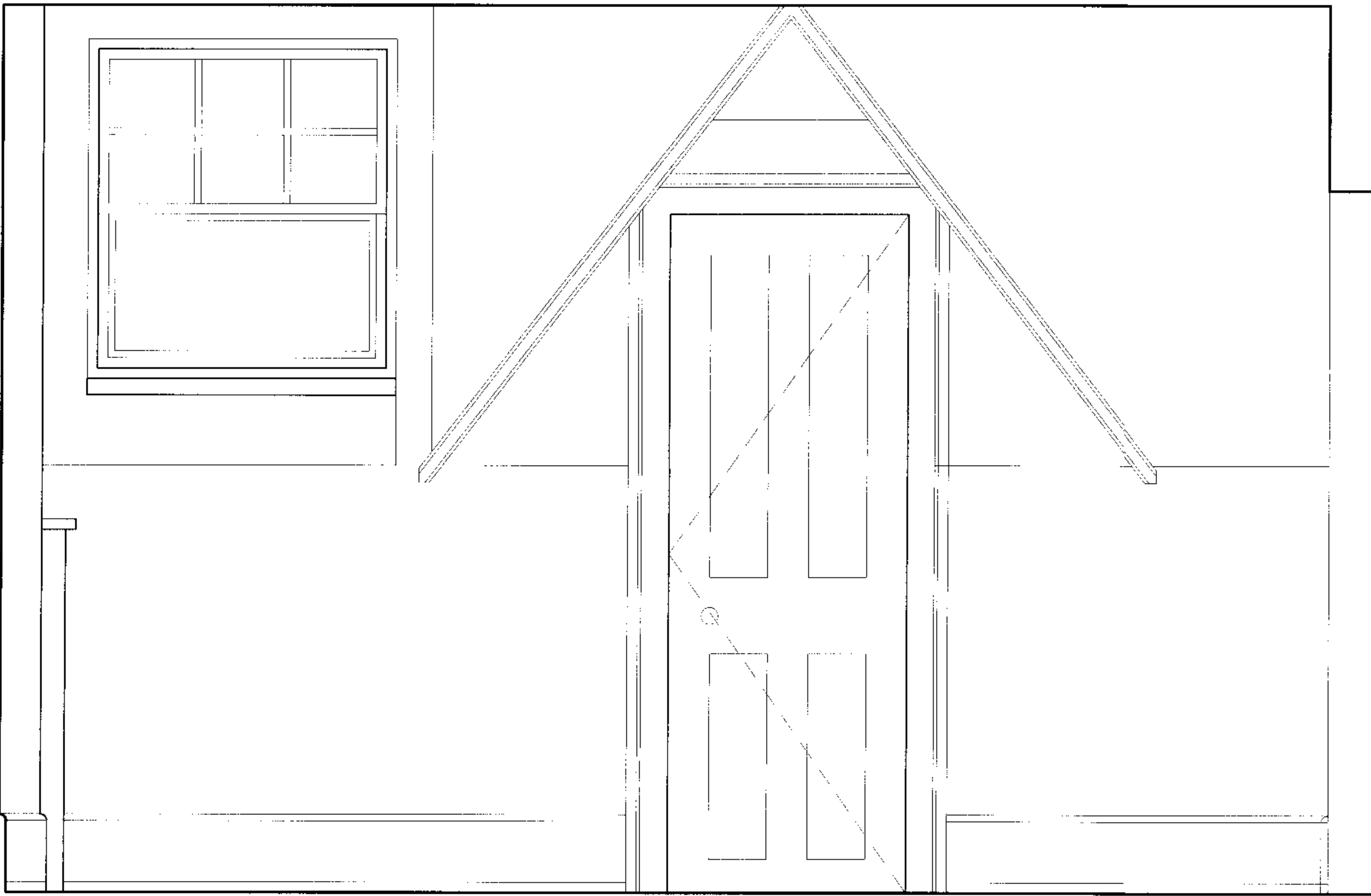
ELEVATION C
