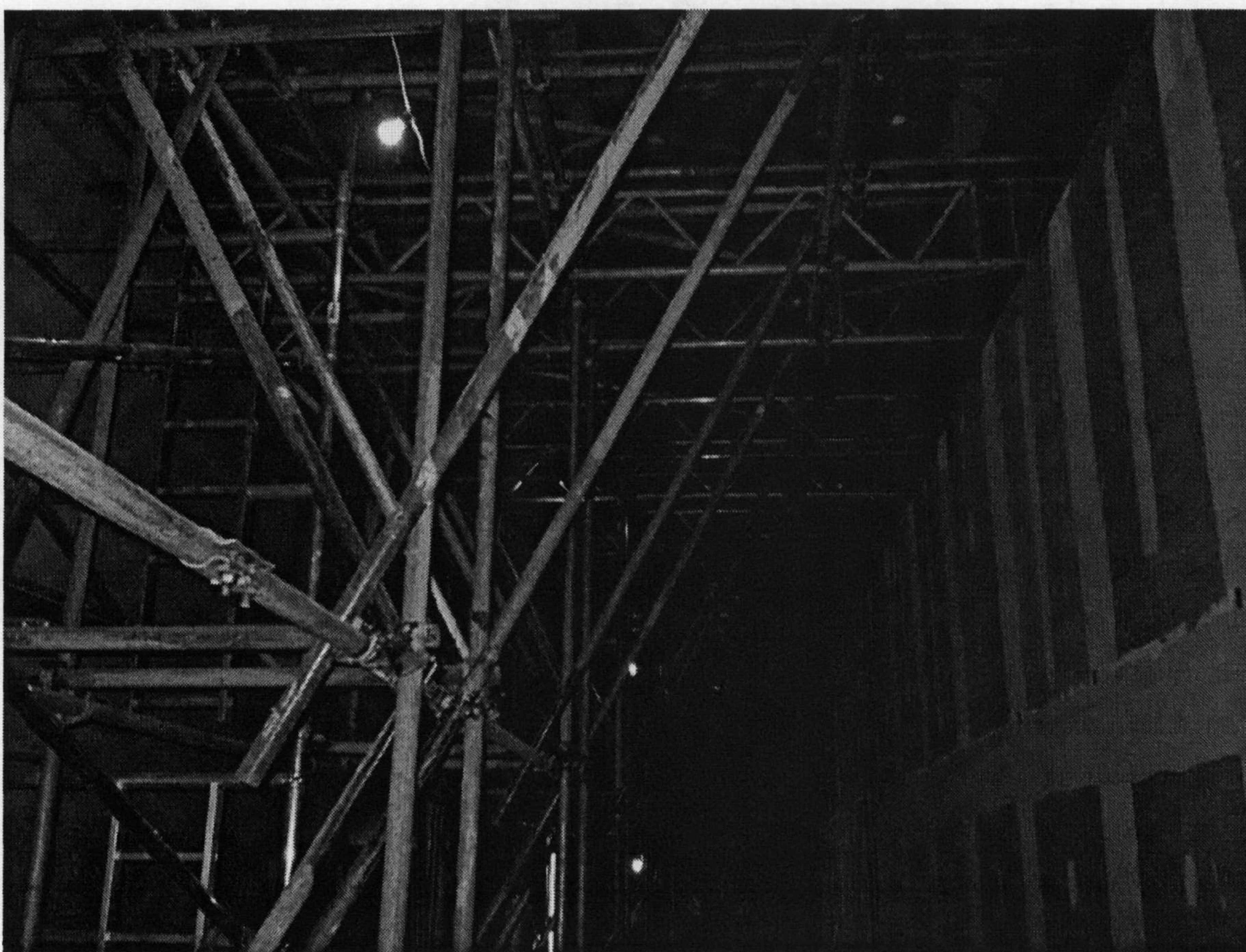
Photograph 4 Gallery 40 South Wall showing bracing. Scaffolding not supported off walls or fixed to walls.
