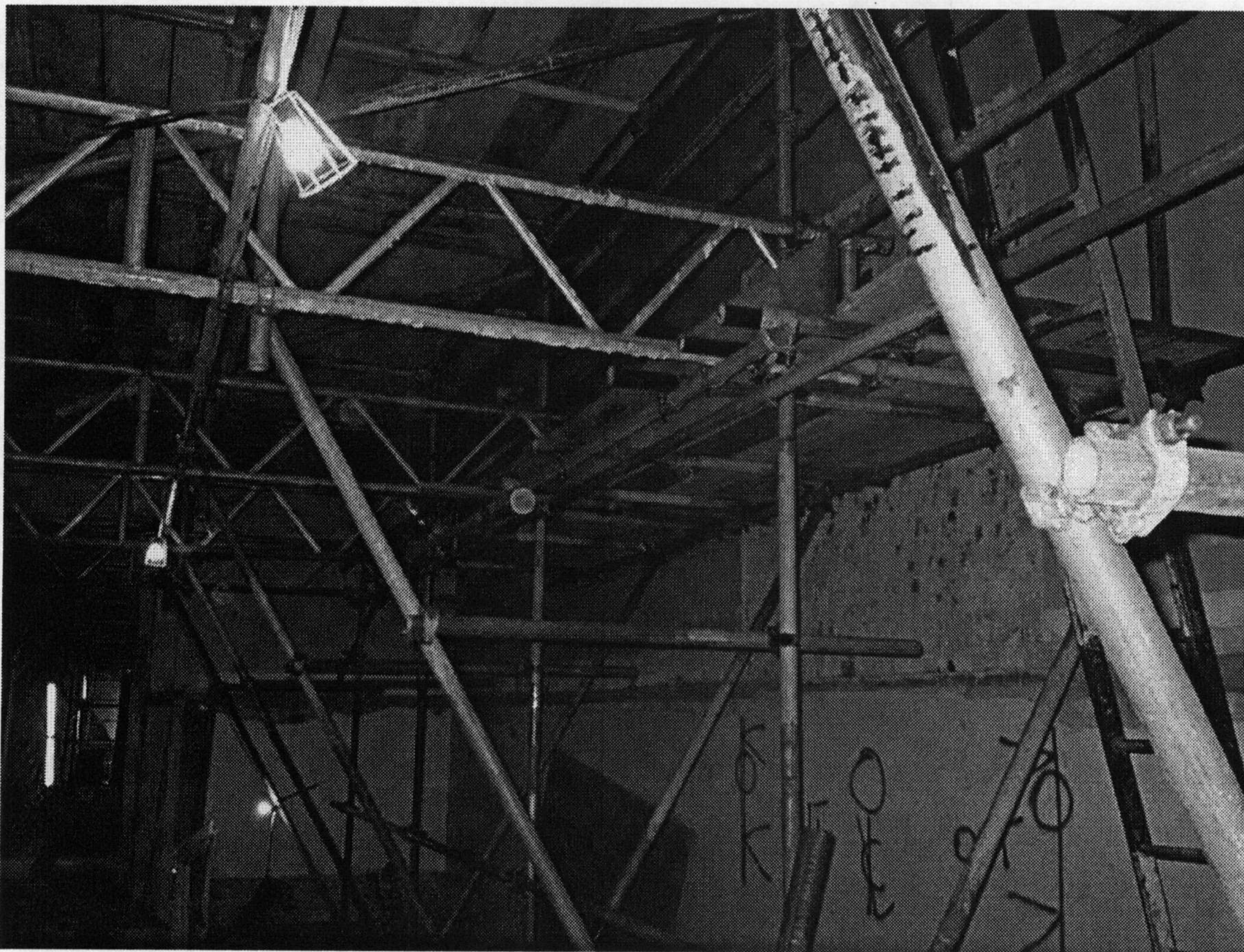
Photograph 2 Gallery 39 North Wall Crash Deck with beams across Gallery. Scaffolding not fixed into walls.
