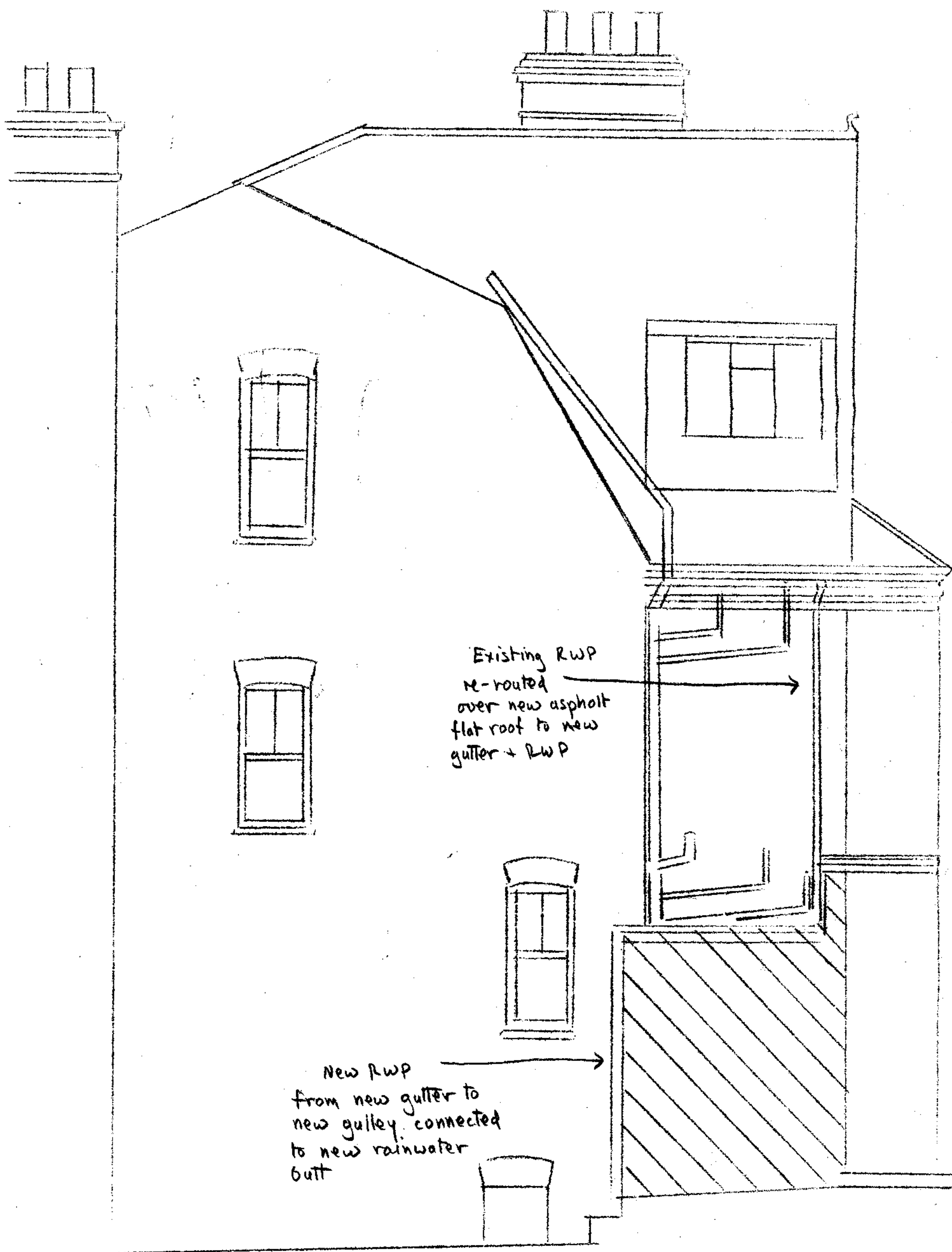
SIDE ELEVATION
