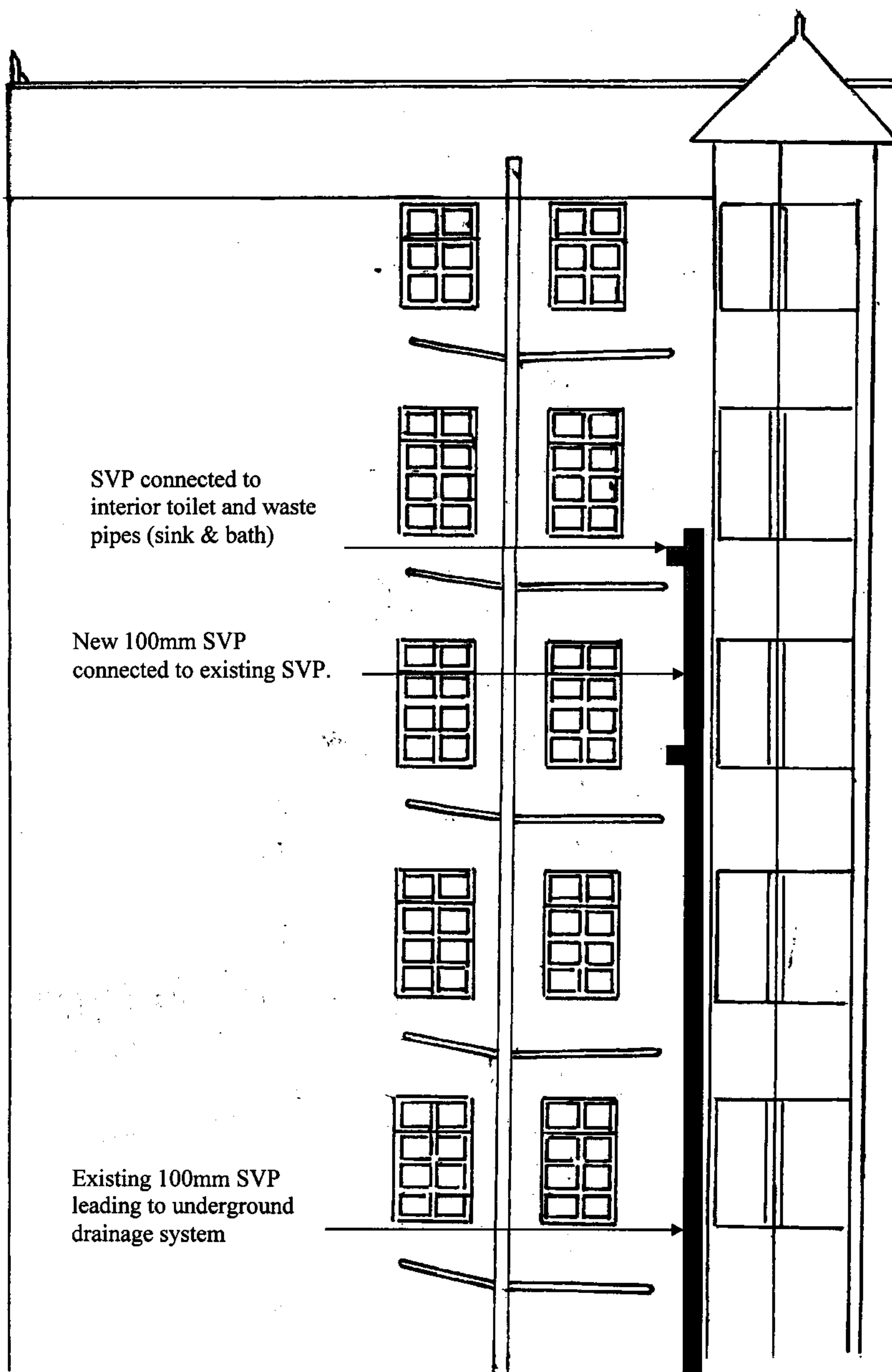
ELEVATION: Figure 01 / Scale 1:50
