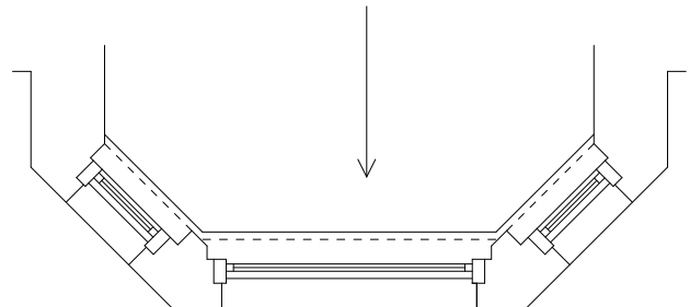
PLAN OF BAY WINDOW
