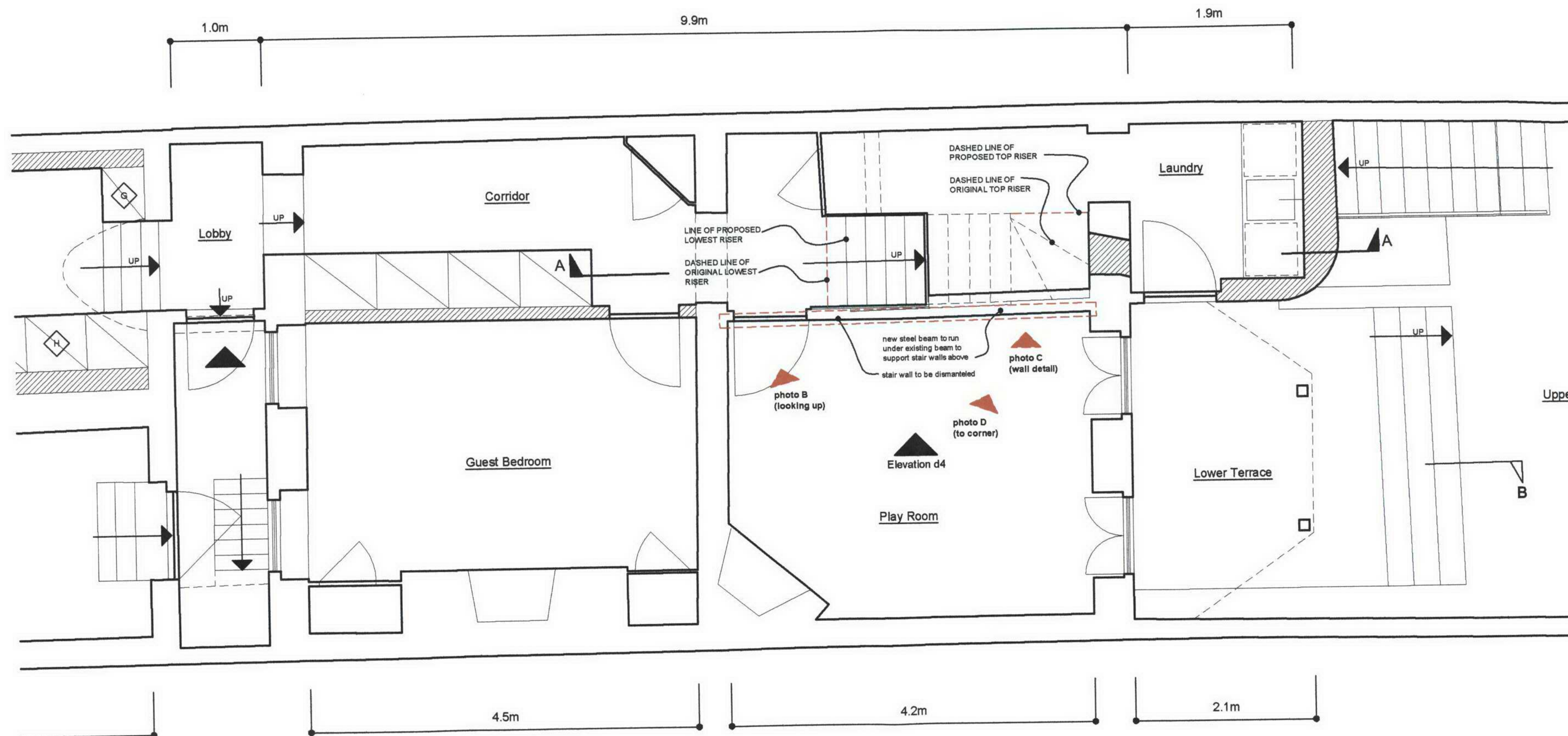
Lower Ground Floor Plan Original & Proposed Stair Positions
