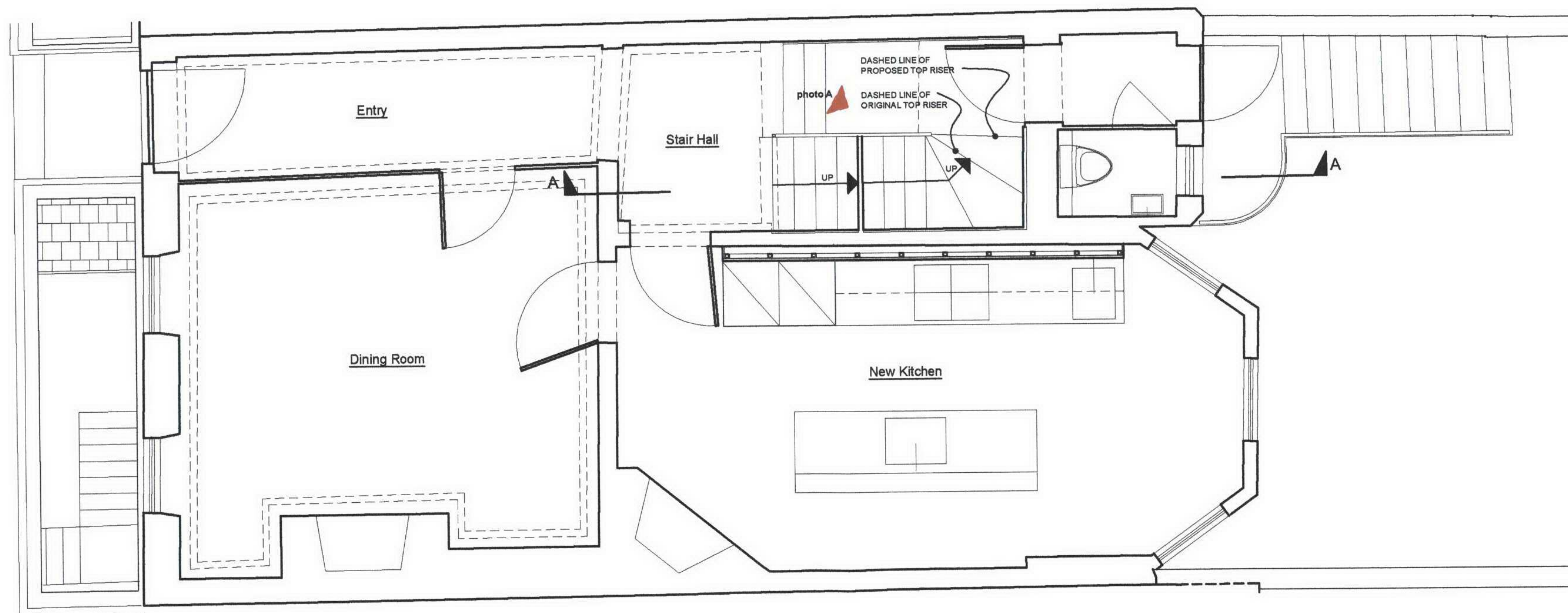
Ground Floor Plan Original & Proposed Stair Positions
