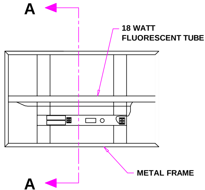
INTERNAL VIEW WITH FRONT PANEL REMOVED
