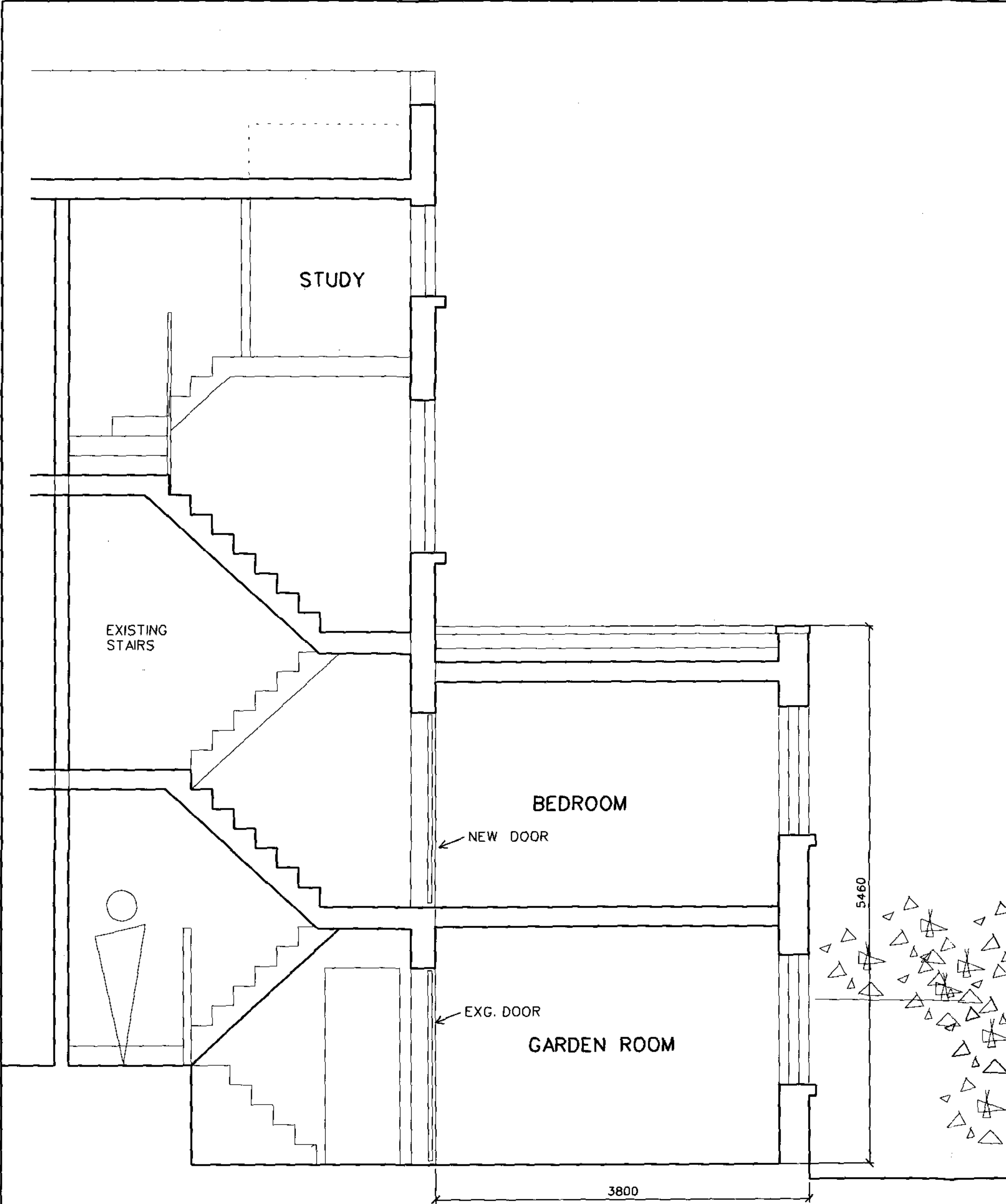
PROPOSED SECTION A-A - THROUGH EXTENSION
