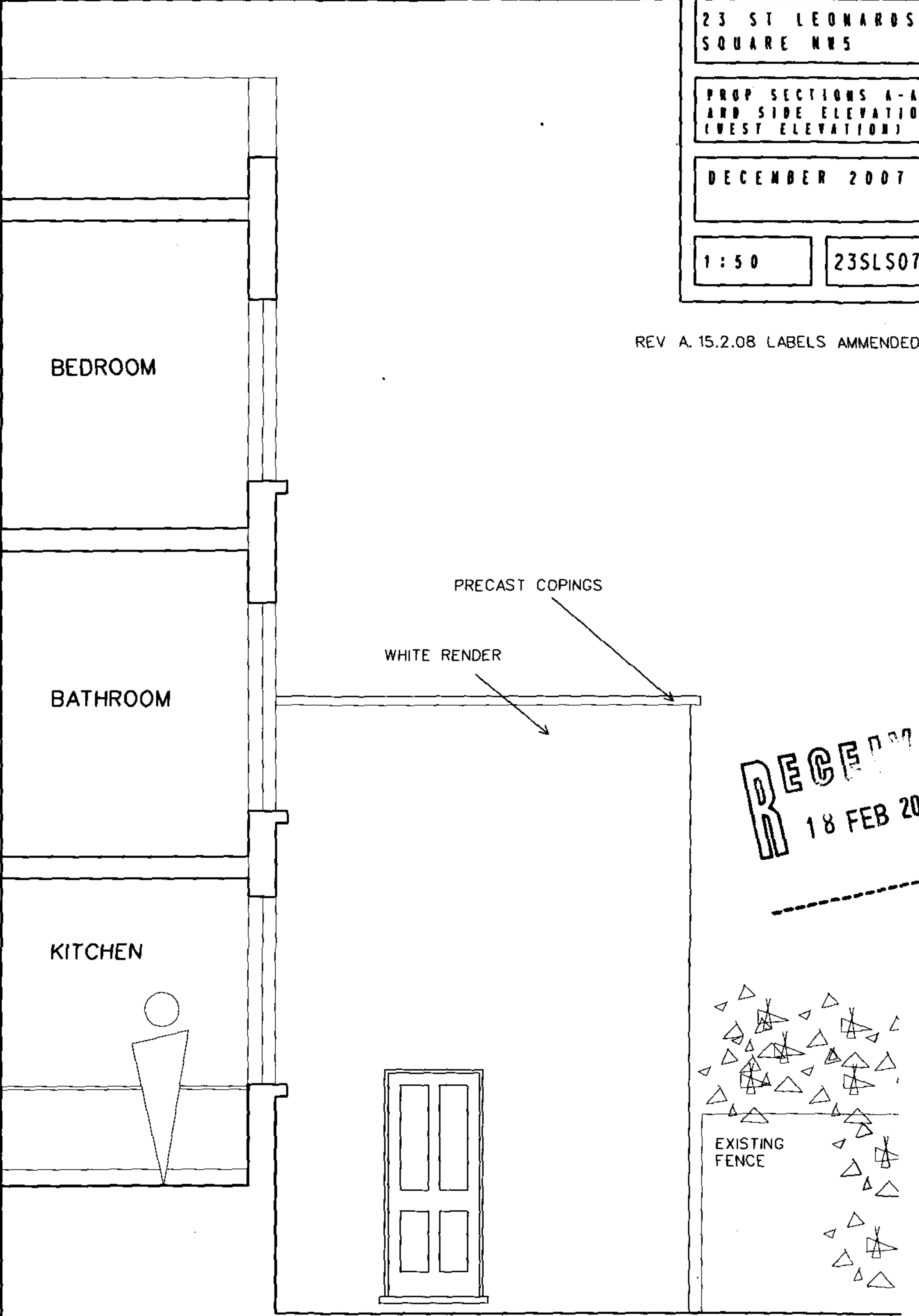
PROPOSED WEST ELEVATION & SECTION THROUGH KITCHEN
