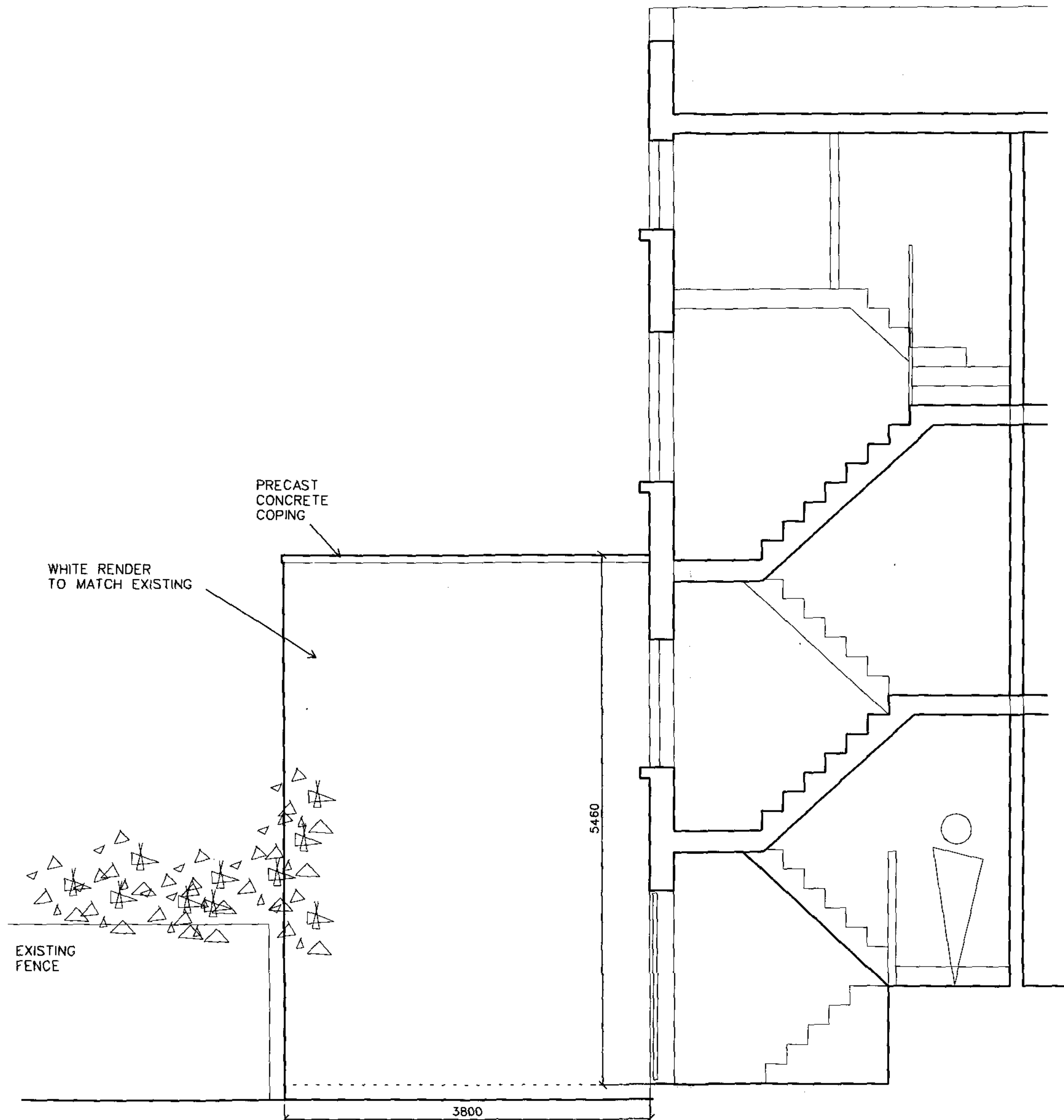
PROPOSED SIDE (EAST) ELEVATION AND SECTION THROUGH NO. 22
