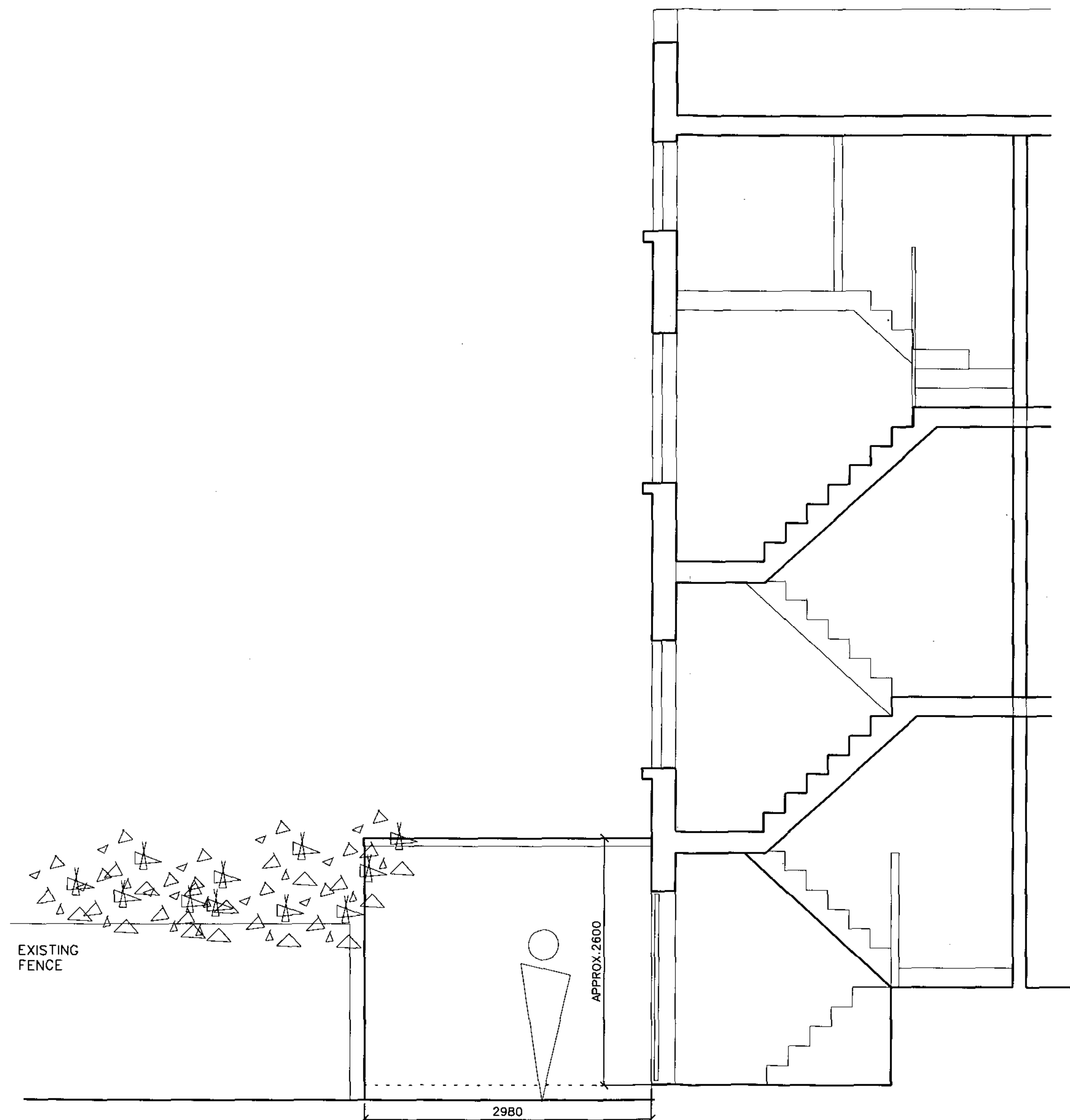
EXISTING SIDE (EAST) ELEVATION AND SECTION THROUGH NO. 22
