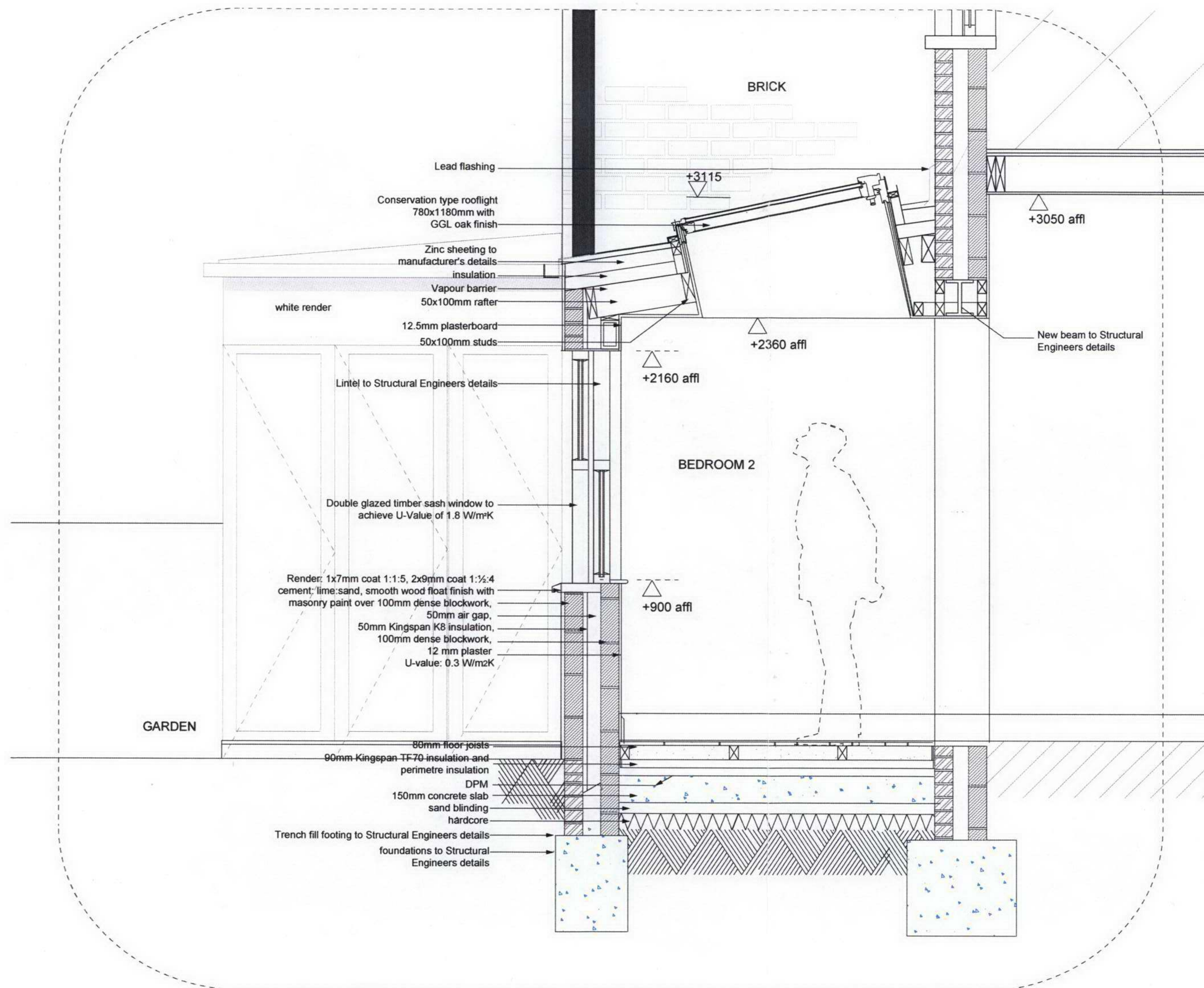
PROPOSED BEDROOM EXTENSION- SECTION BB SCALE 1:25@A3
