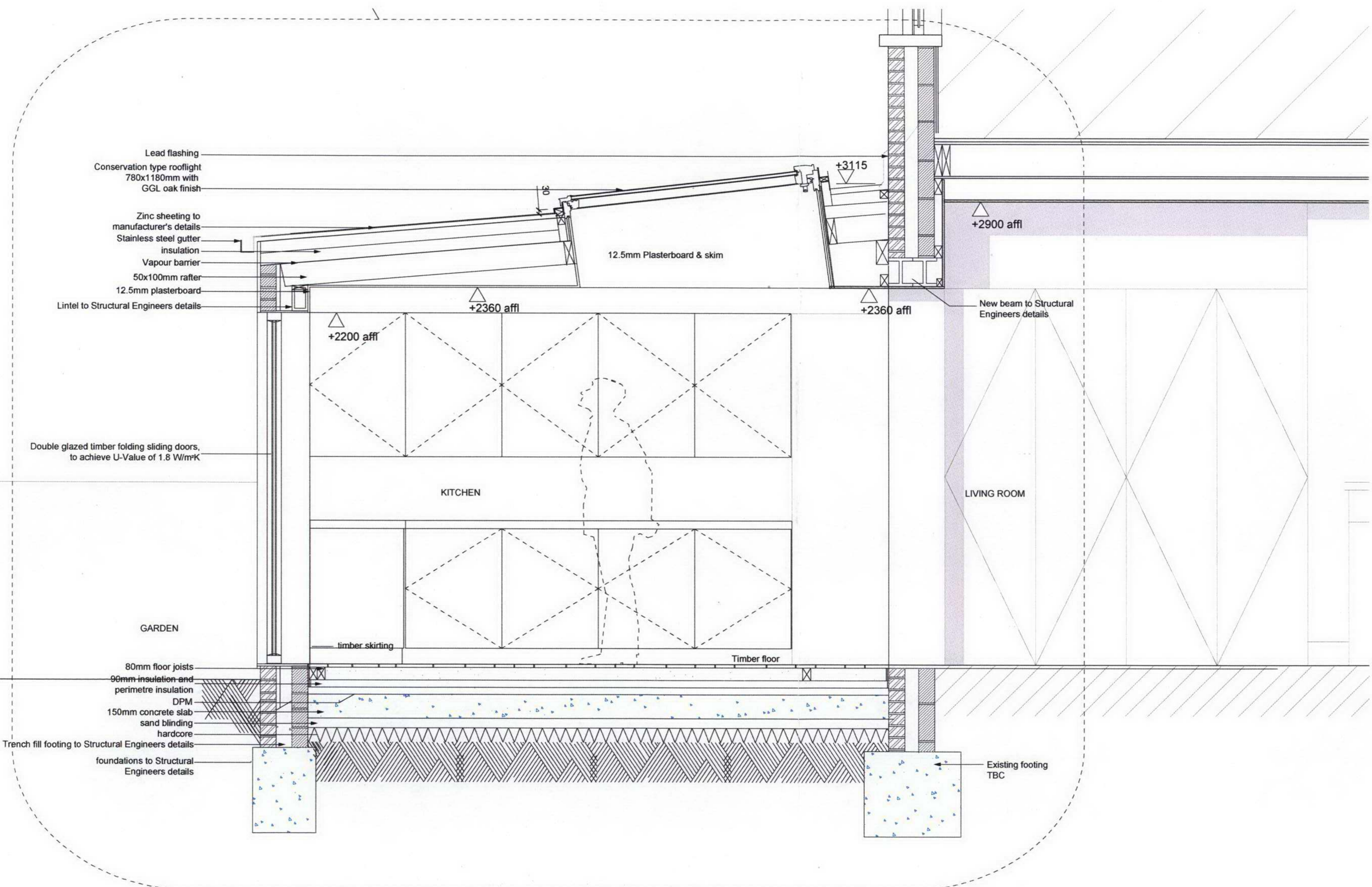
PROPOSED KITCHEN EXTENSION- SECTION AA SCALE 1:25@A3
