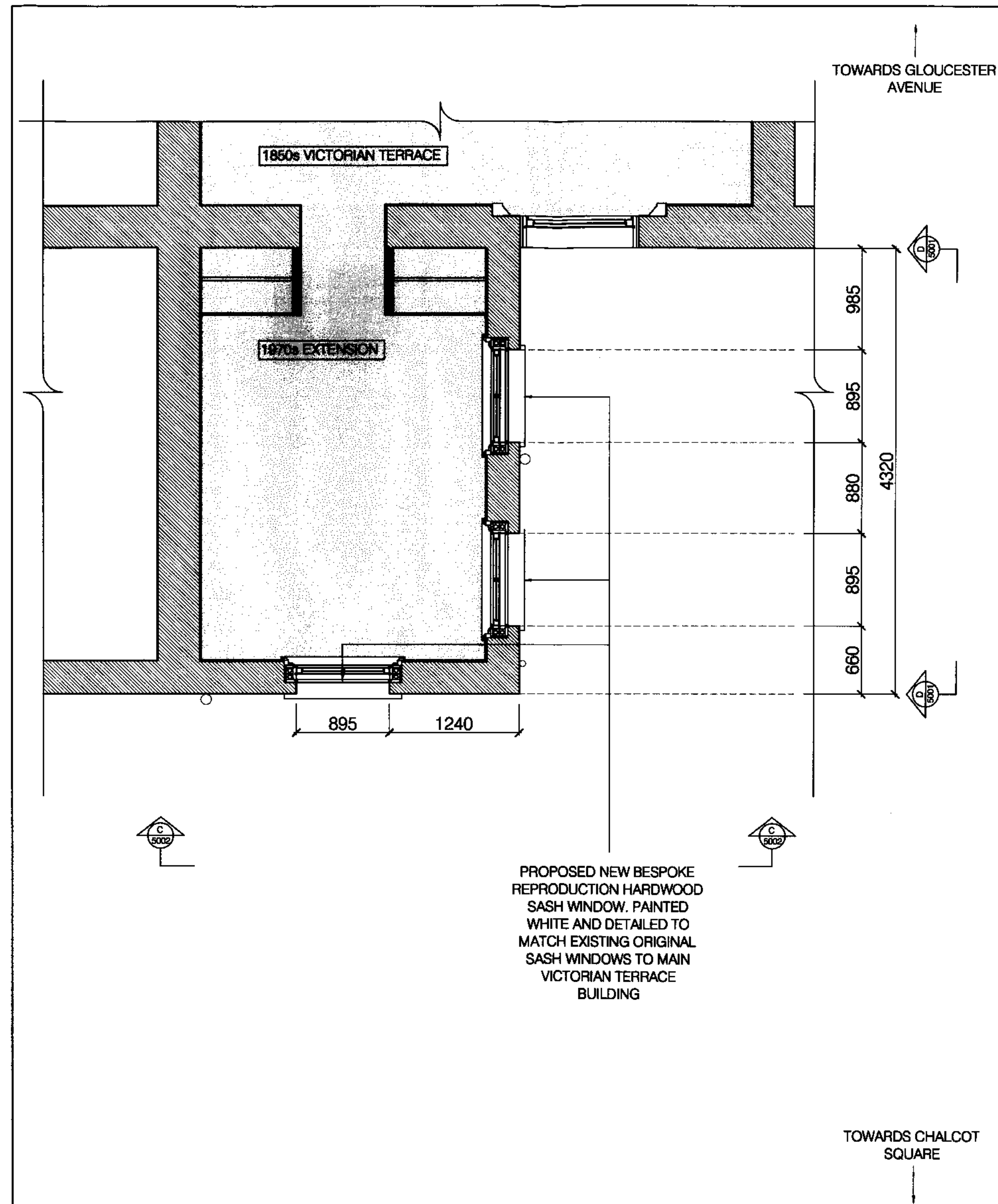
02 EXTENSION PLAN SHOWING PROPOSED WINDOW TYPE, SIZE AND POSITION SCALE: 1:50 @ A3
