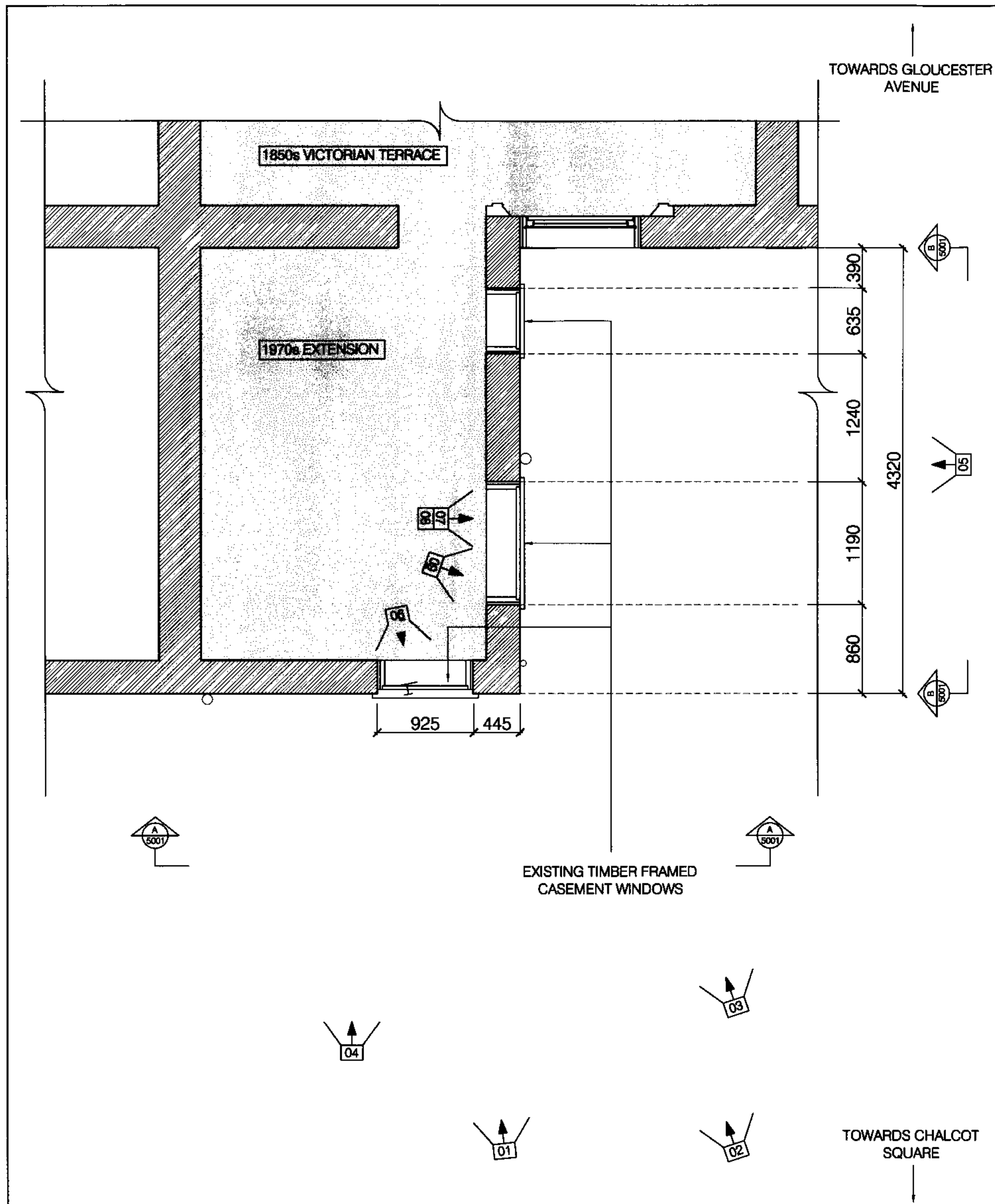
01 EXTENSION PLAN SHOWING EXISTING WINDOW TYPE, SIZE AND POSITION SCALE: 1:50 @ A3
