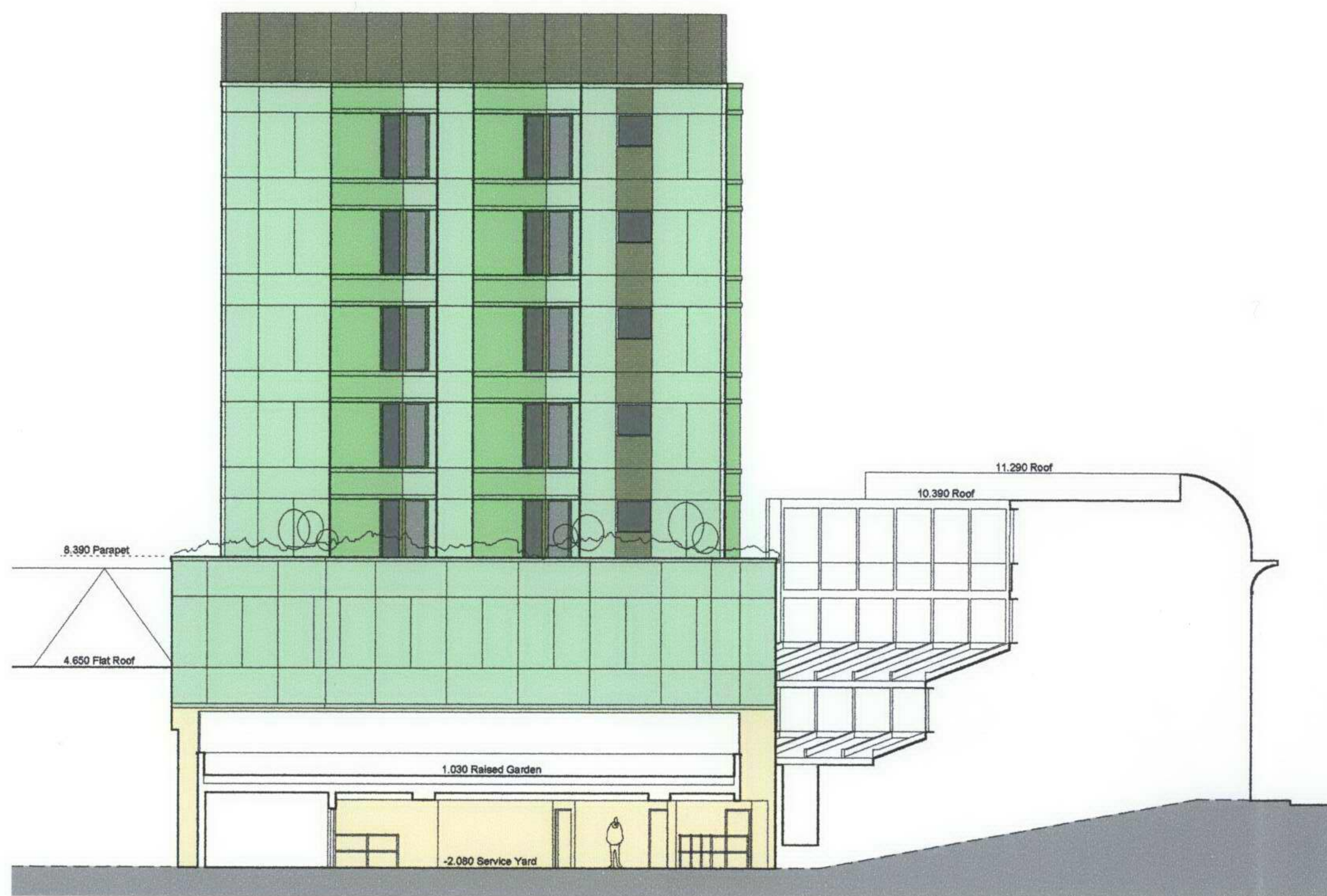
ELEVATION FROM 1-11 HAWLEY CRESCENT Scale 1:100
