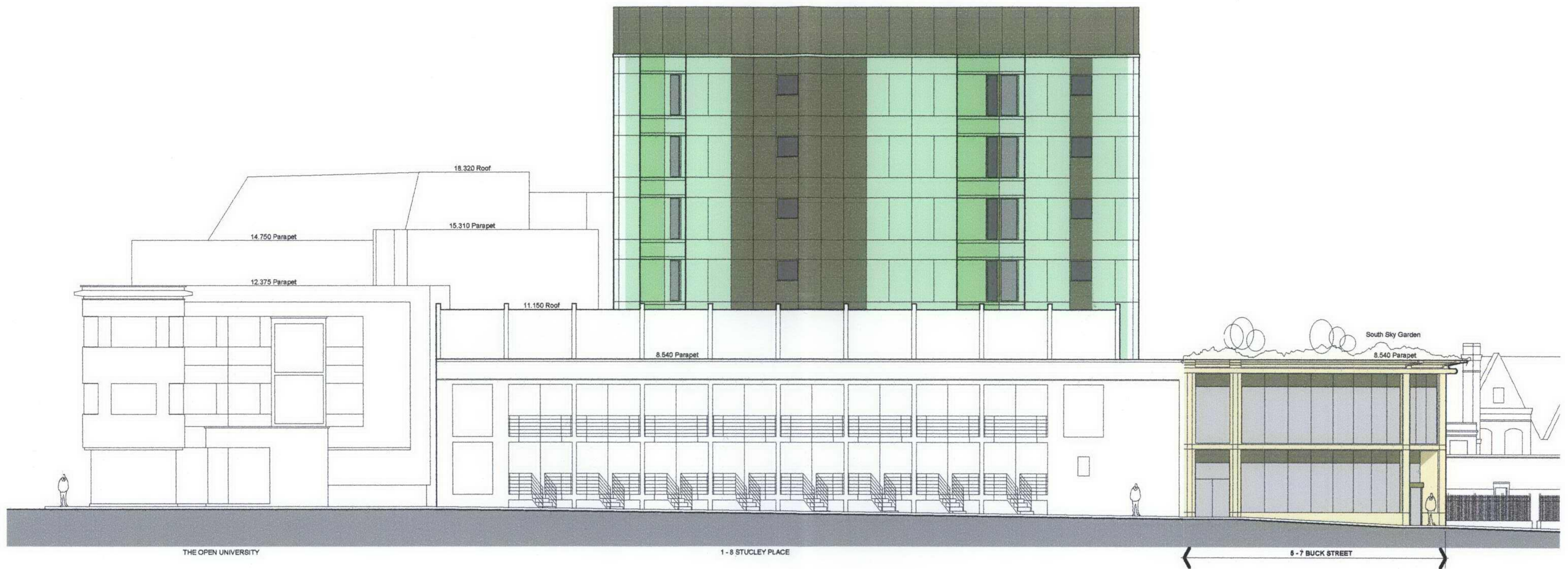
ELEVATION FROM STUCLEY PLACE Scale 1:200
