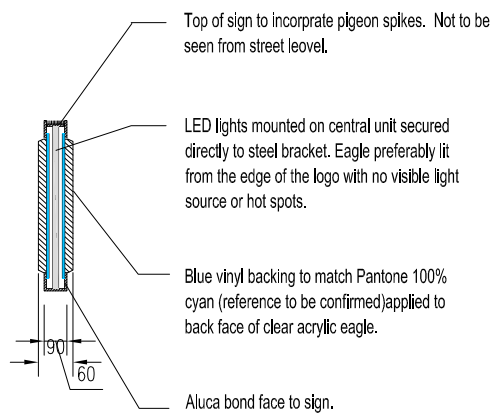
Section 1:20
