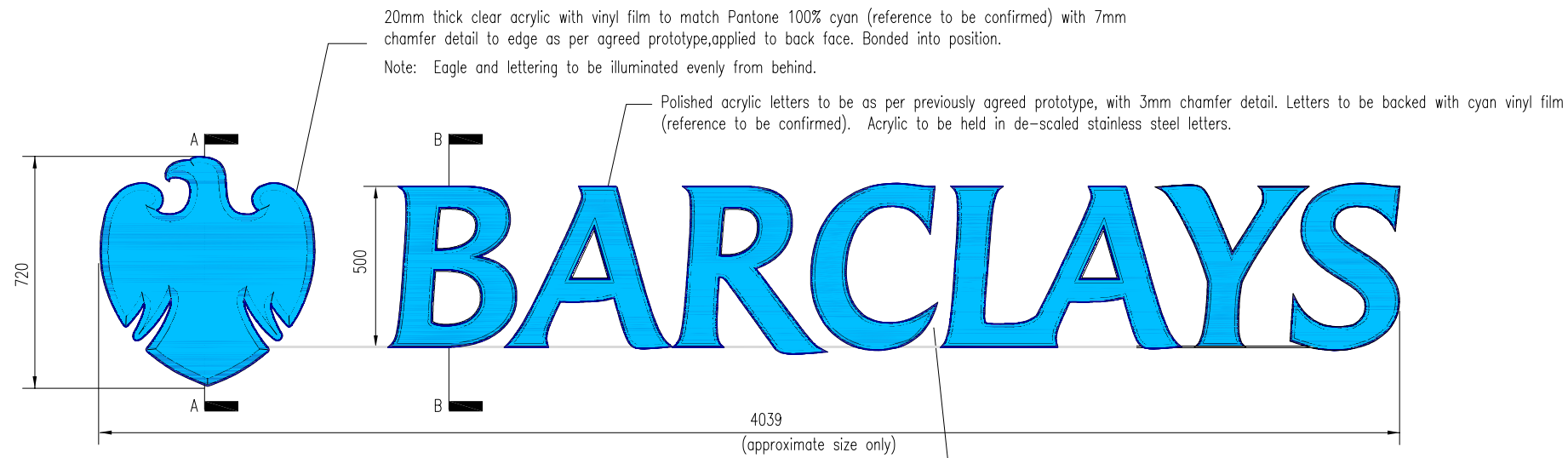
Front Elevation 1:20 500mm Lettering
