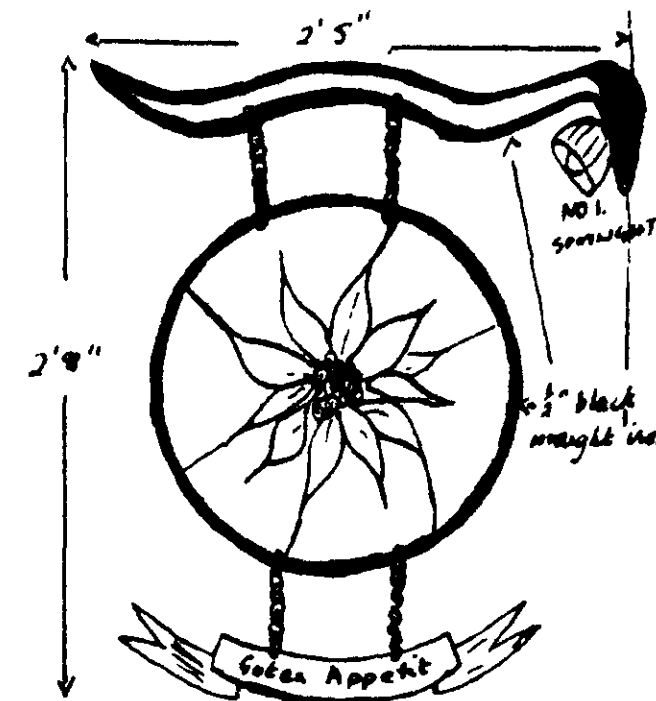
Measurement of Proposed Sign and Situation of Spotlight Scale: 1/10" = 1'
