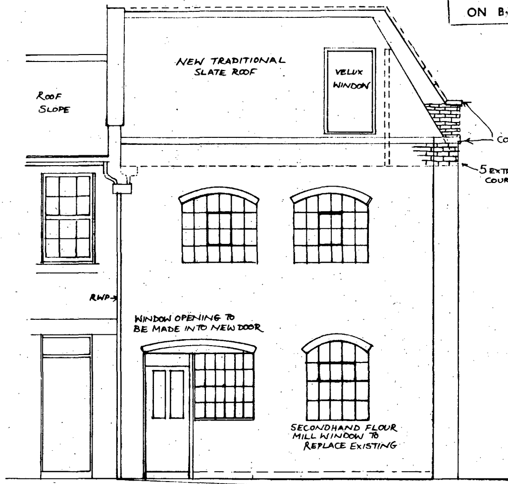
SIDE ELEVATION
