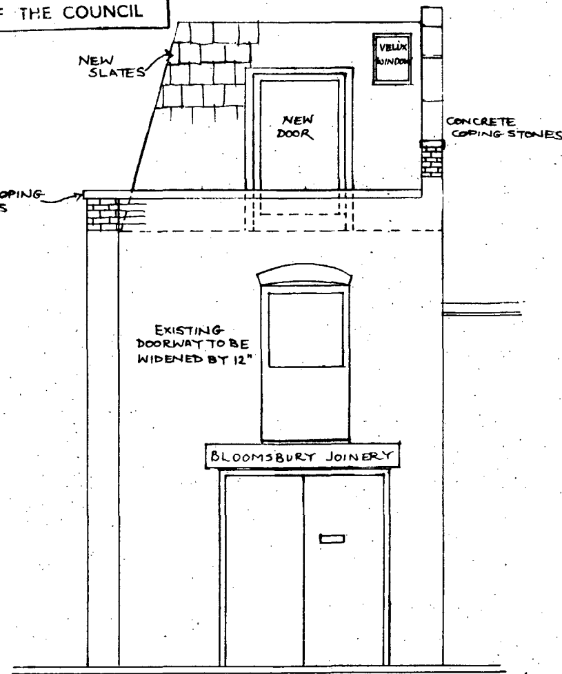
FRONT ELEVATION
