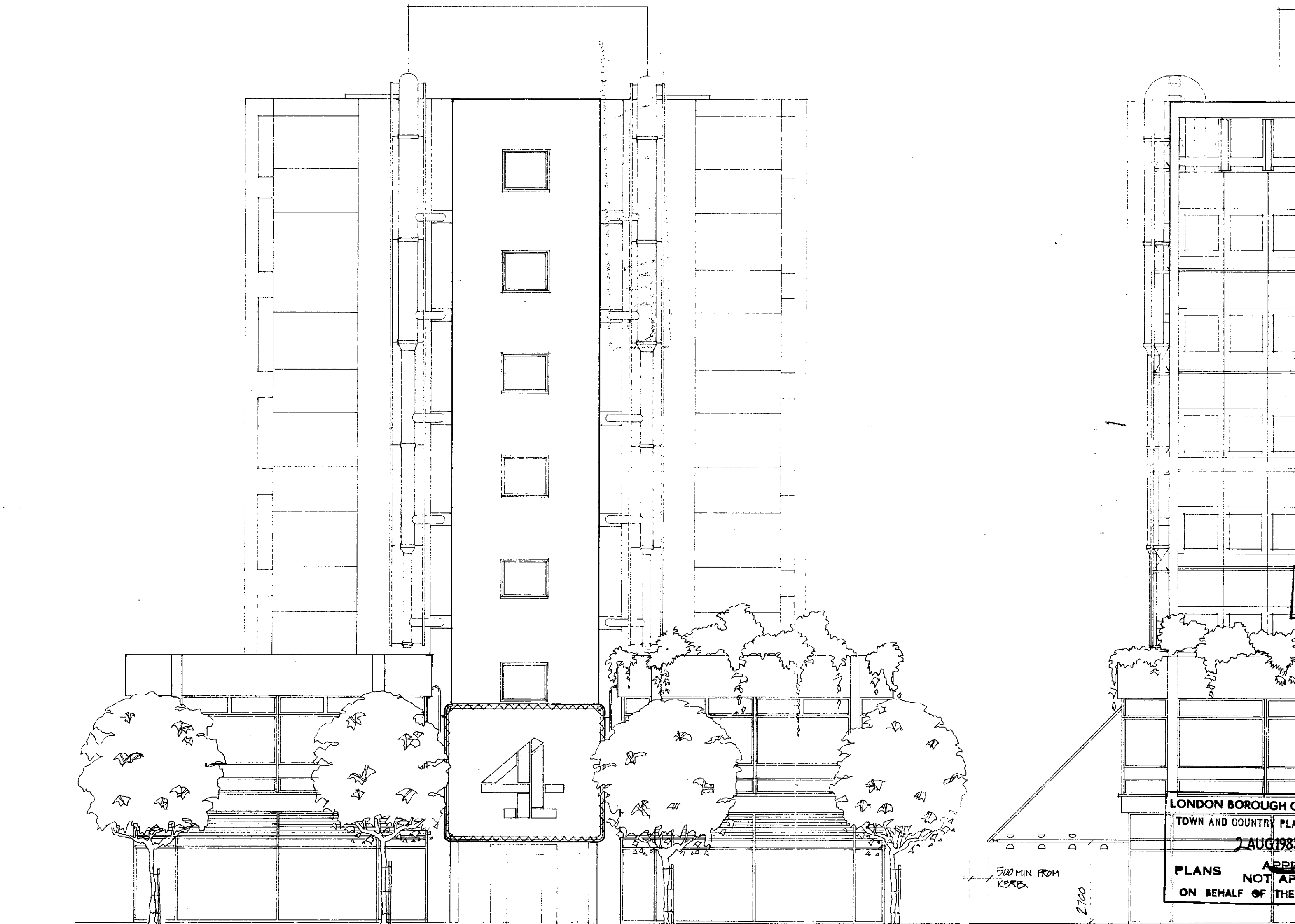
CHARLOTTE STREET ELEVATION
