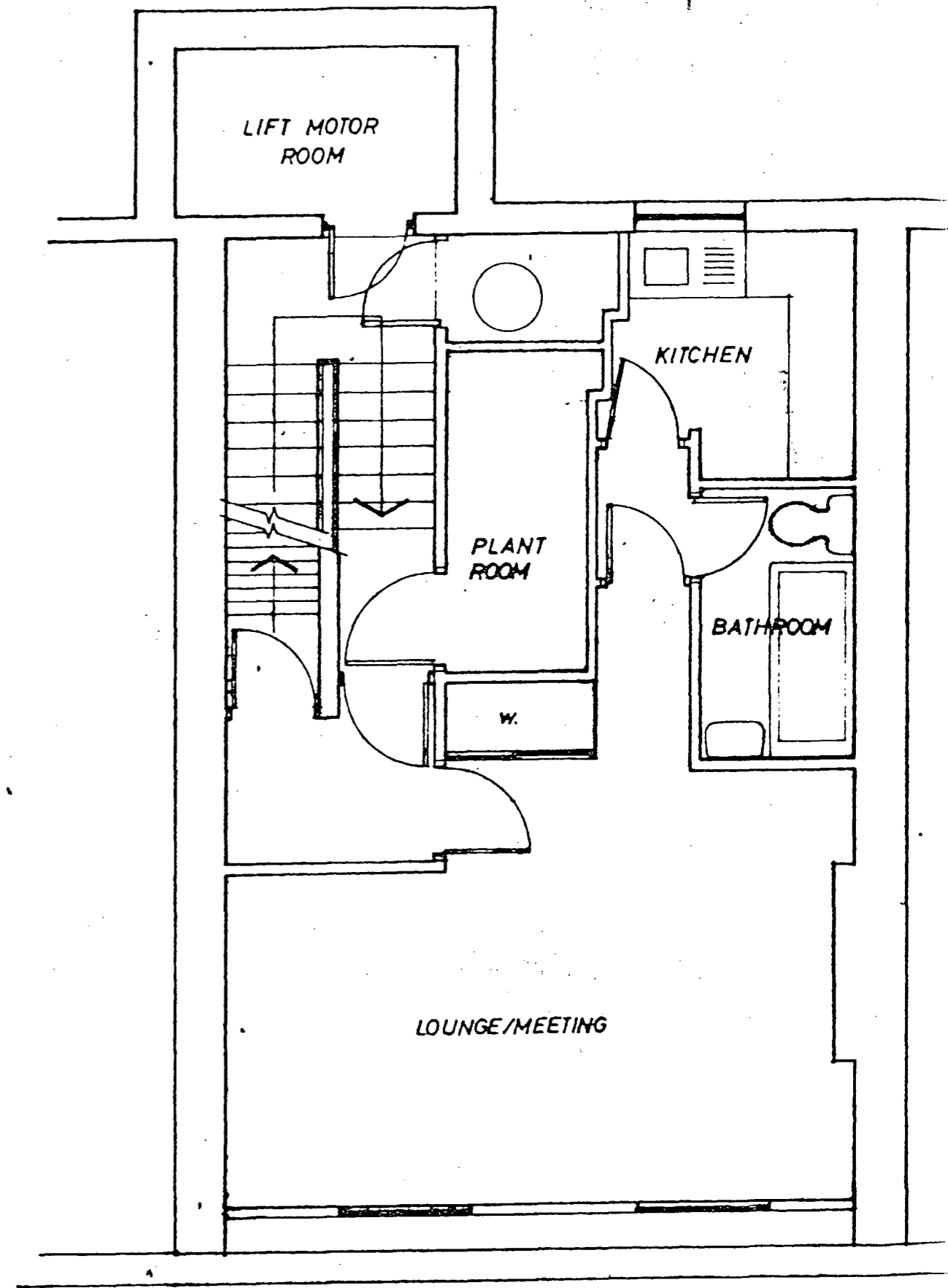
FOURTH FLOOR PLAN AS EXISTING
