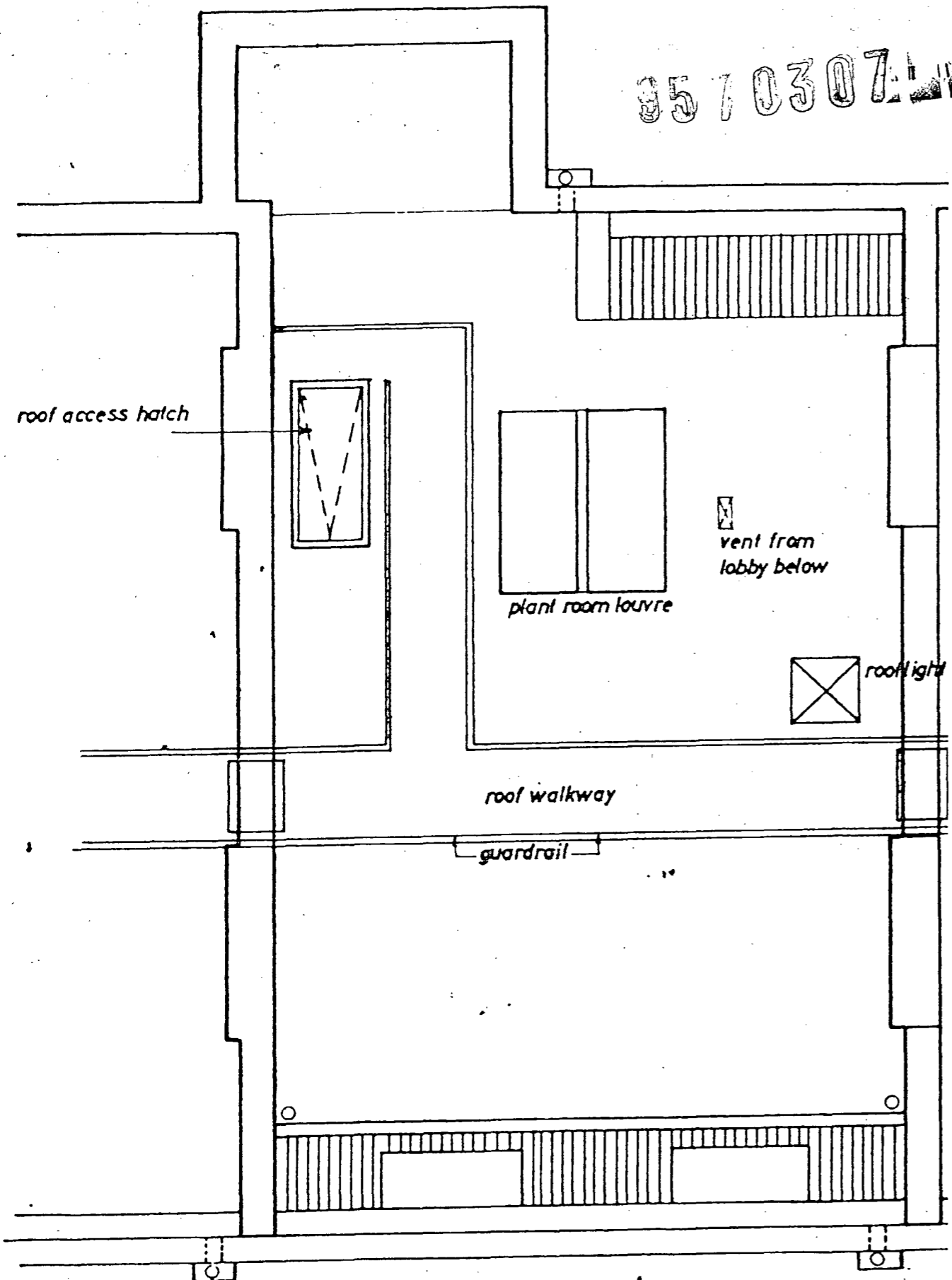
ROOF PLAN AS EXISTING
