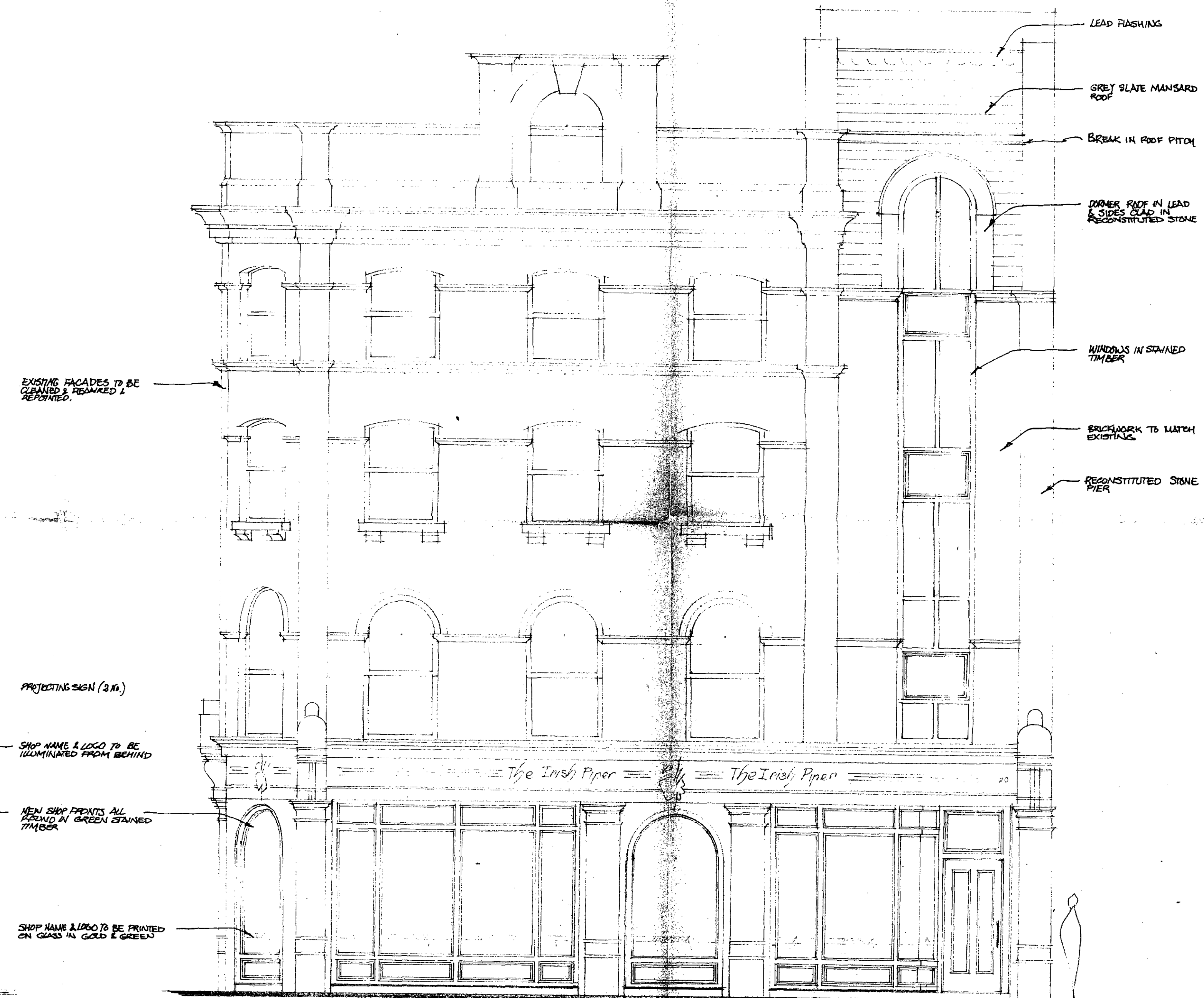
elevation to BLOOMSBURY ST.
